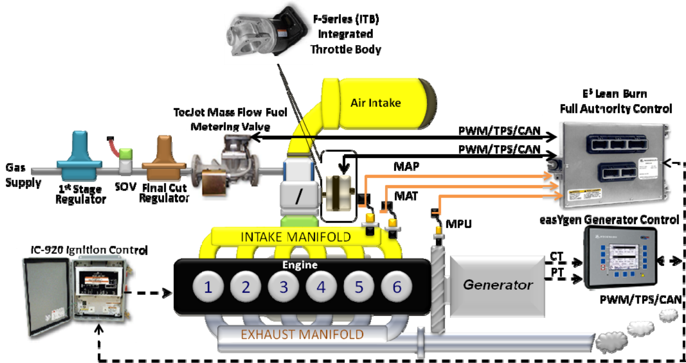
E 3 Lean Burn Full Authority Control System Configuration
