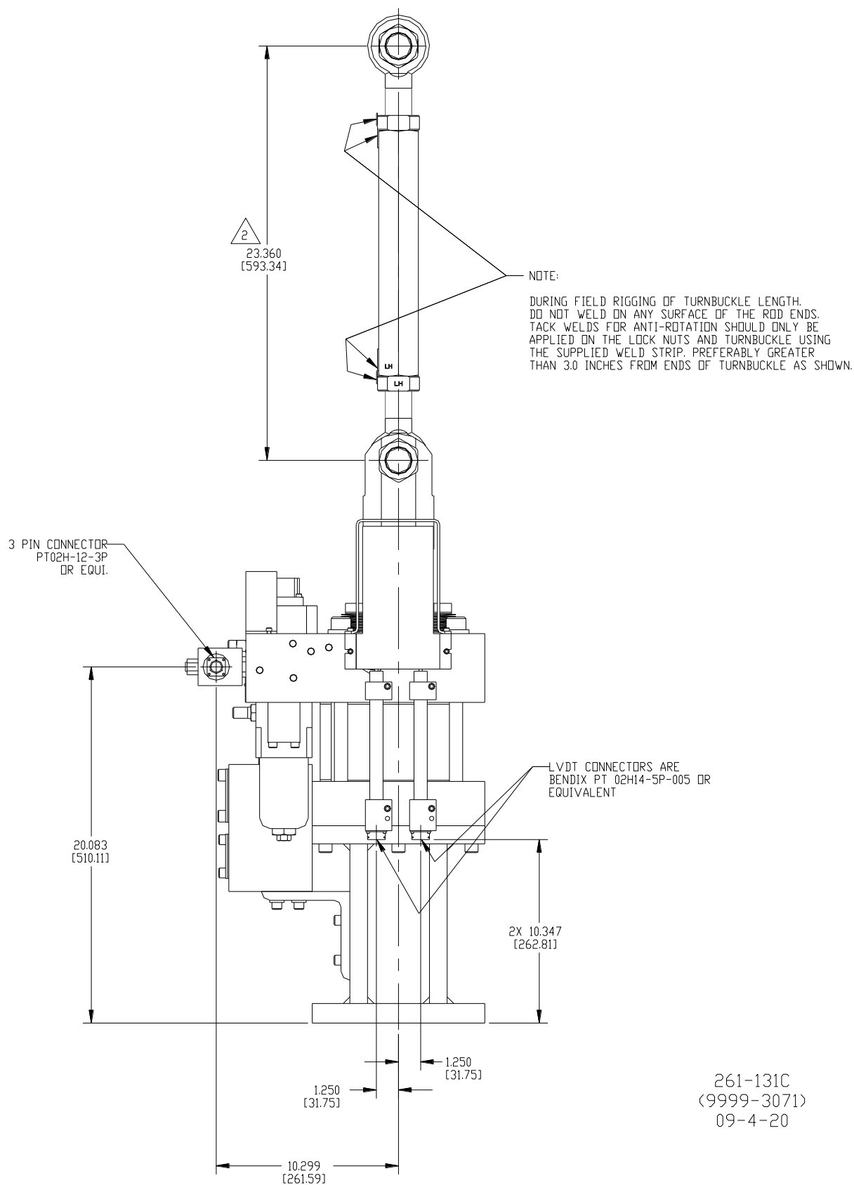
Figure 1-8c. 7F IGV Actuator with Electric Trip (right side view)
