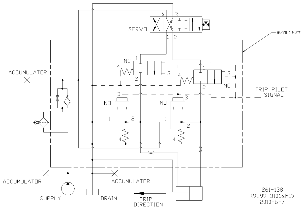
Figure 1-11. IGV Hydraulic Schematic, High Pressure Trip Option (Hydraulic Trip System)
