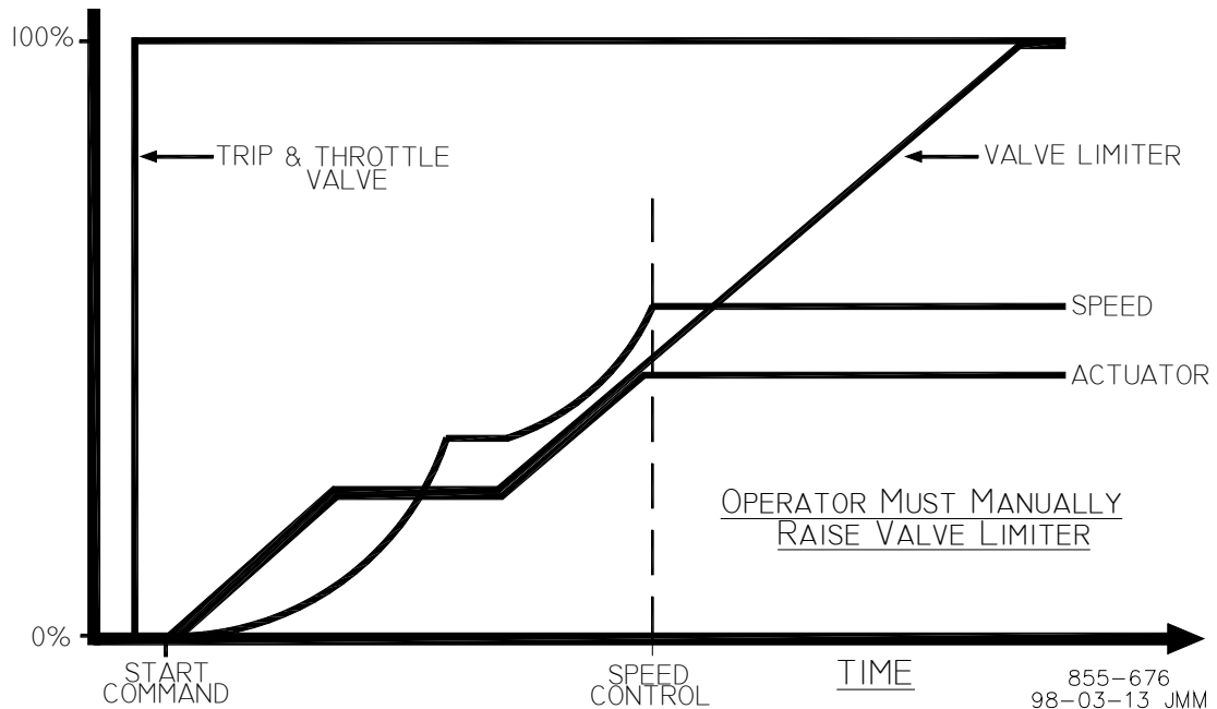
Figure 2-15. Semiautomatic Start Mode Example
