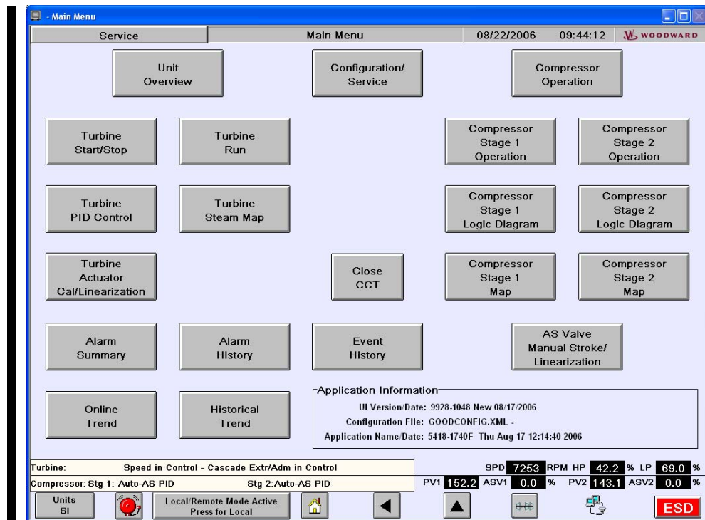
Figure 5-1. Main Menu Screen
