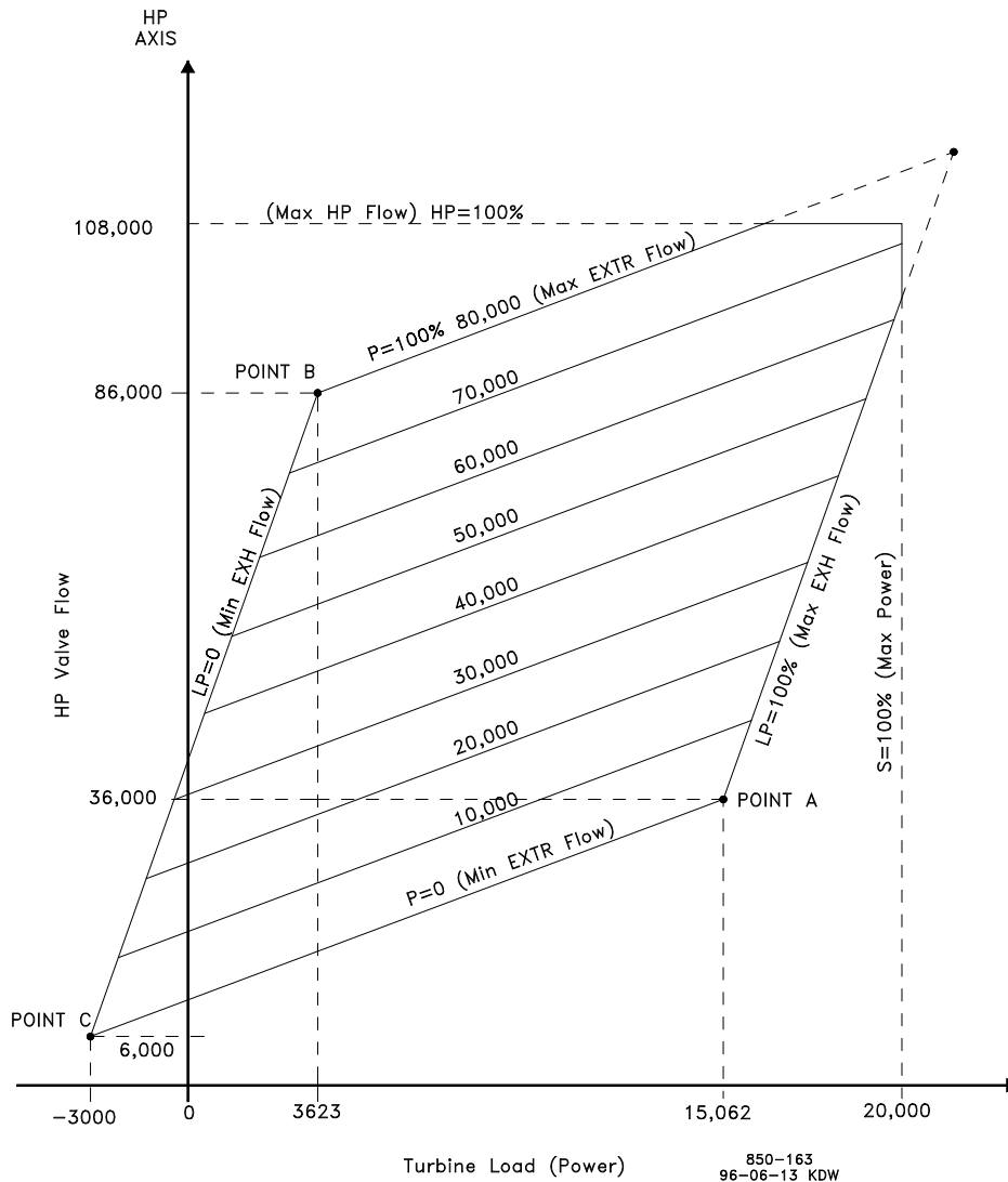
Figure 4-9. Typical Extraction Steam Map
