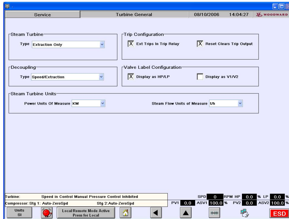
Figure 4-2. Turbine General Configuration Screen
