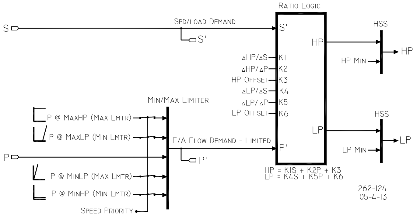
Figure 2-10. Coupled HP &amp; LP Mode
