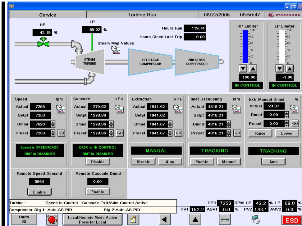
Figure 5-7. Turbine Run Screen
