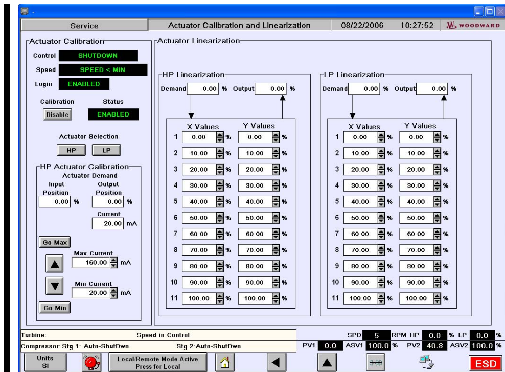
Figure 5-17. Turbine Actuator Cal/Linearization Screen
