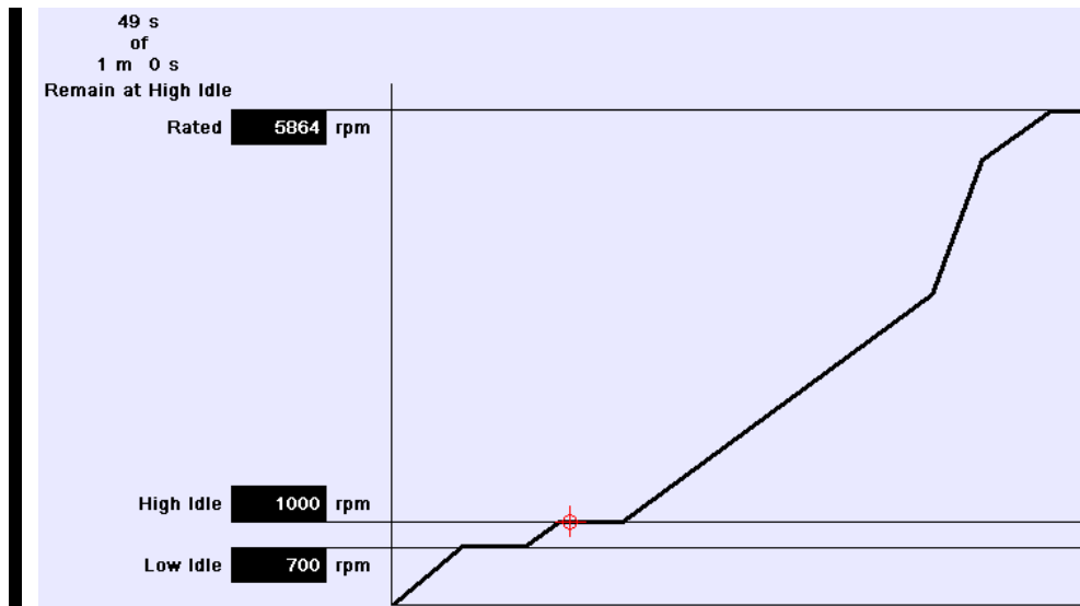
Figure 5-5. Turbine Start Screen Startup Diagram
