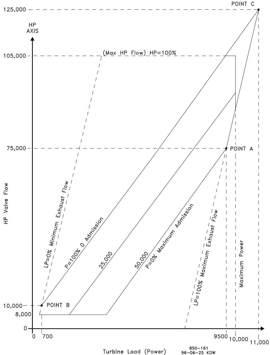
Figure 4-10. Typical Admission Steam Map
