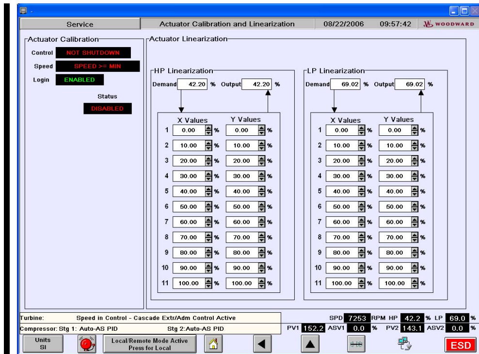
Figure 5-16. Turbine Actuator Cal/Linearization Screen
