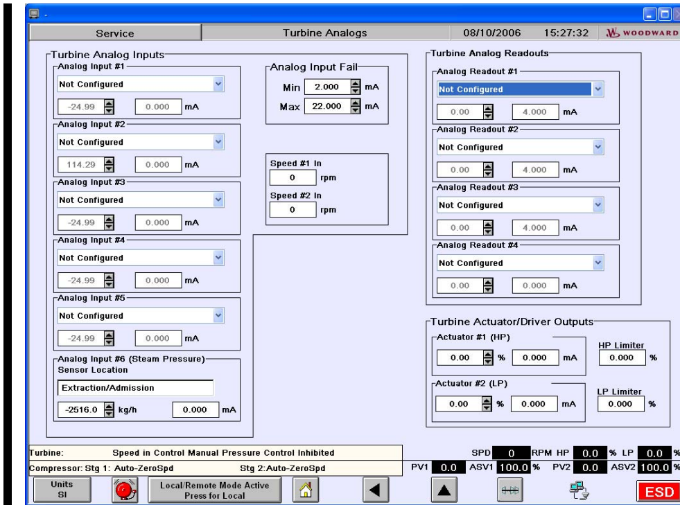
Figure 4-16. Turbine Analogs Configuration Screen
