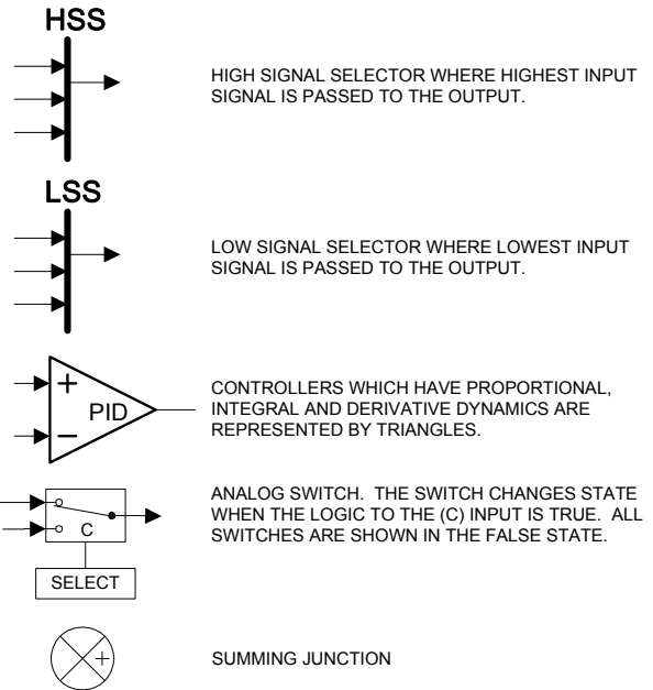
Figure 2-1. Overview of 505CC-2 Control Functionality Notes
