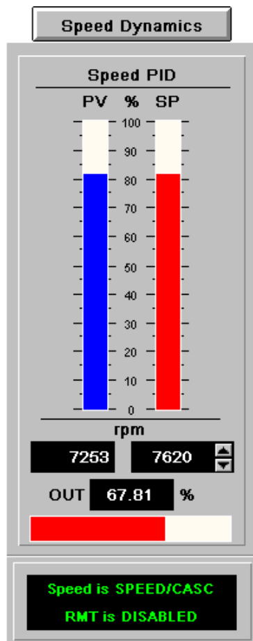
Figure 5-13. Turbine PID Control Screen
