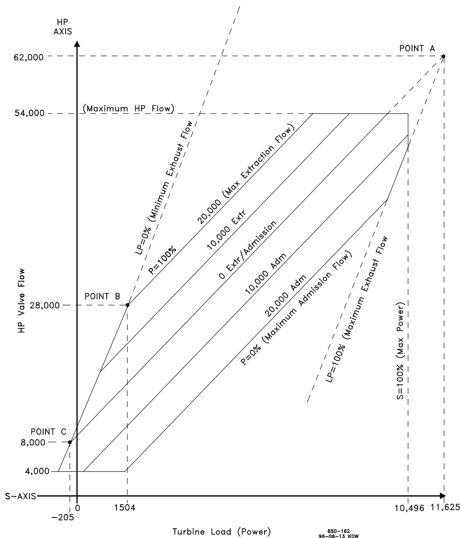
Figure 4-11. Typical Extraction/Admission Steam Map
