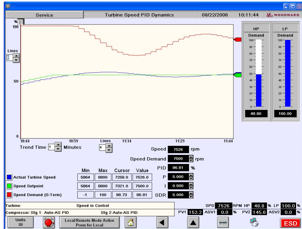
Figure 5-14. Turbine Speed Dynamics Tuning Screen
