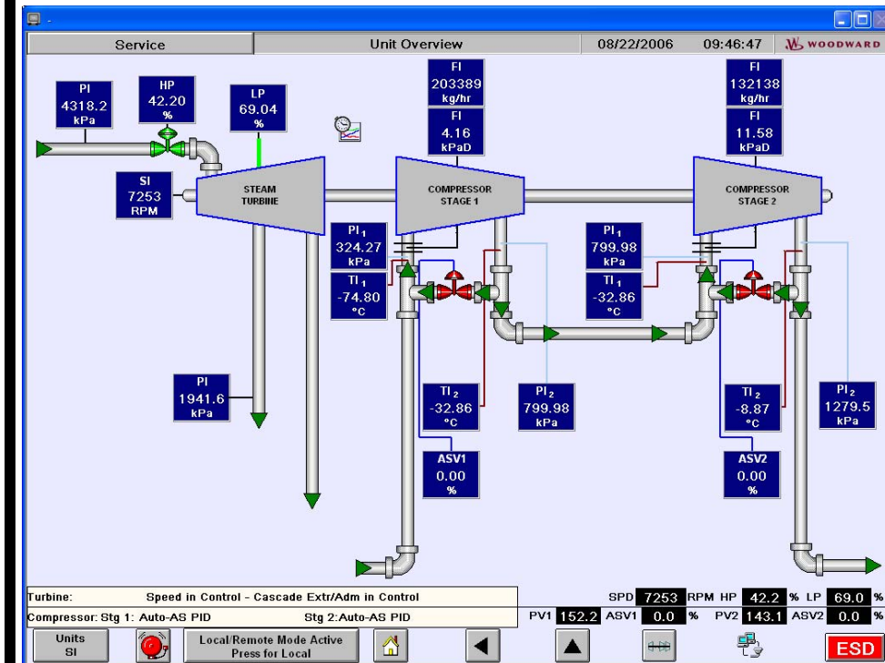
Figure 5-2. Unit Overview Screen
