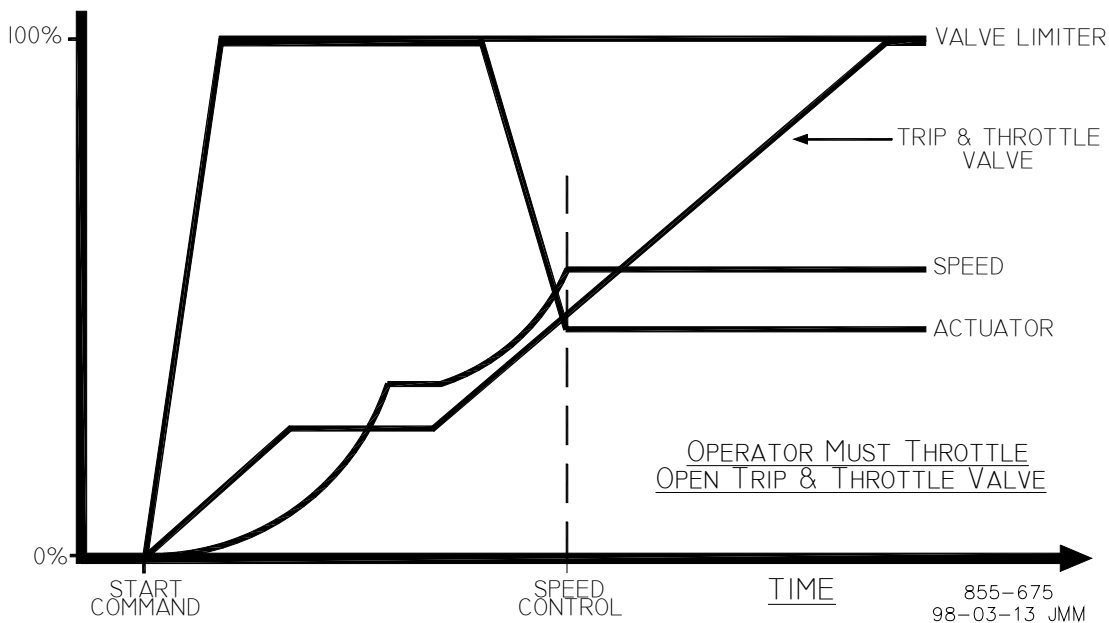
Figure 2-14. Manual Start Mode Example
