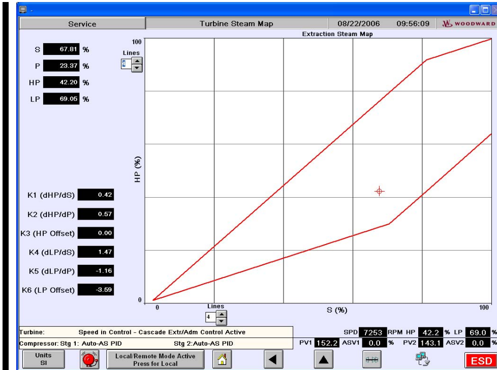
Figure 5-15. Turbine Steam Map Screen
