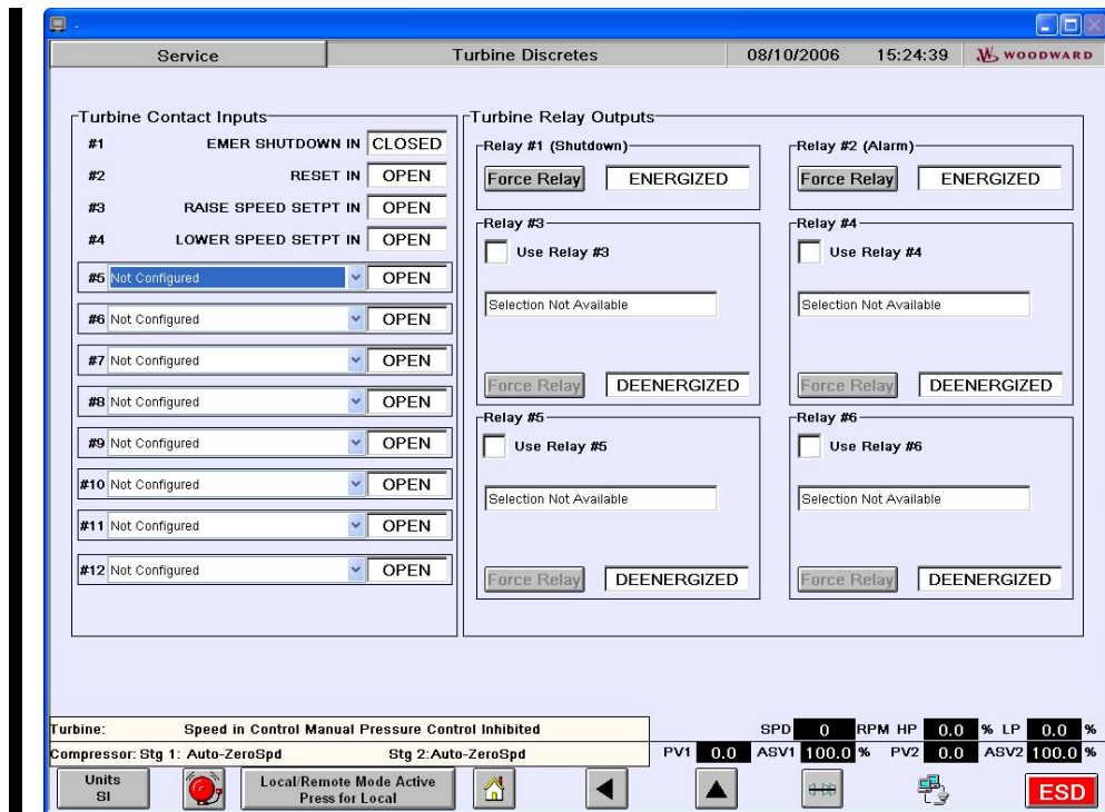
Figure 4-14. Turbine Discretes Configuration Screen
