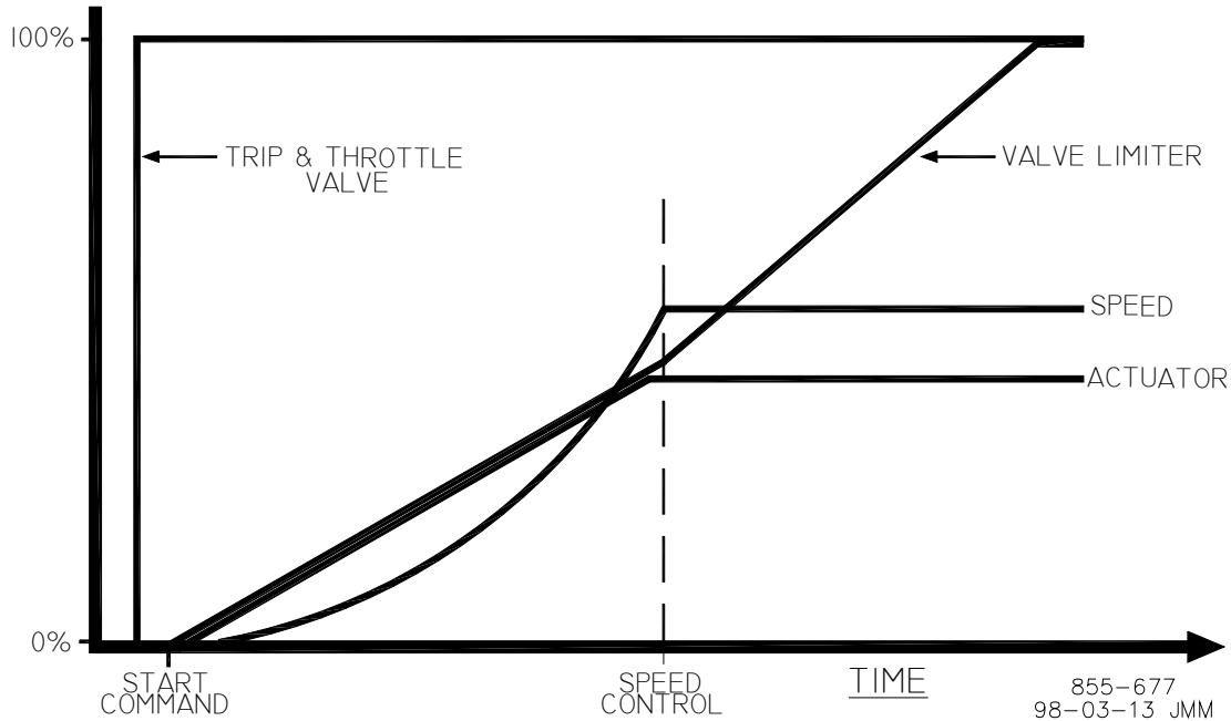
Figure 2-16. Automatic Start Mode Example
