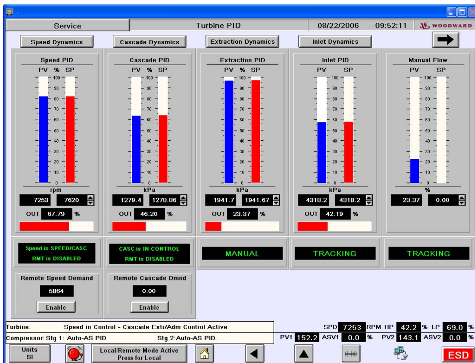
Figure 5-12. Turbine PID Control Screen
