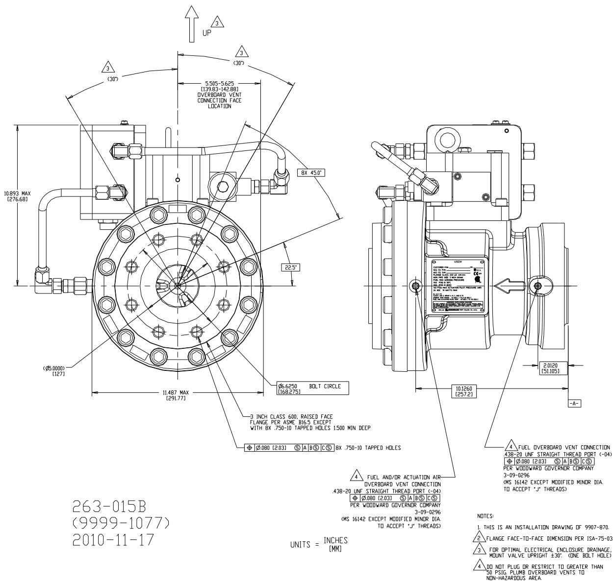
Figure 1-2b. Outline Drawing of 3-Inch USOV
