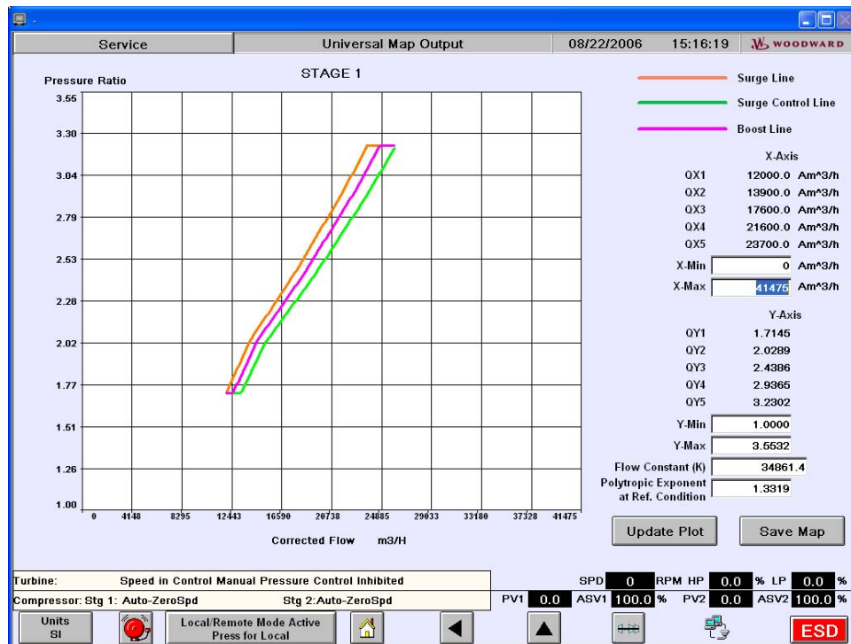
Figure 4-18. Universal Map Output Screen
