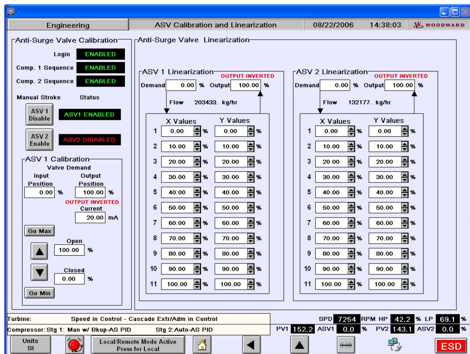
Figure 5-8. Compressor Anti-surge Valve Linearization Screen
