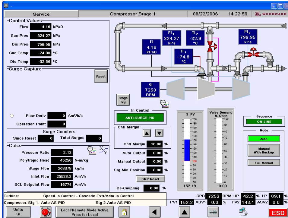
Figure 5-3. Compressor Stage Operation Screen
