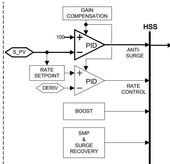
Figure 2-18. Anti-Surge PID
