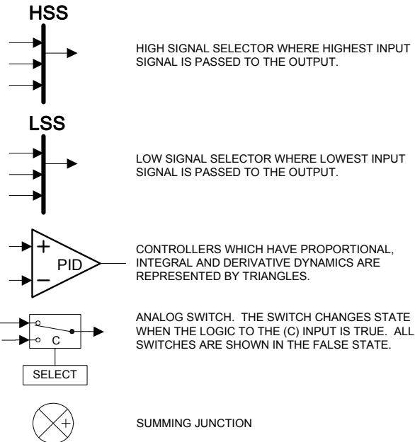
Figure 2-3. Overview of 505CC-2 Functionality Notes
