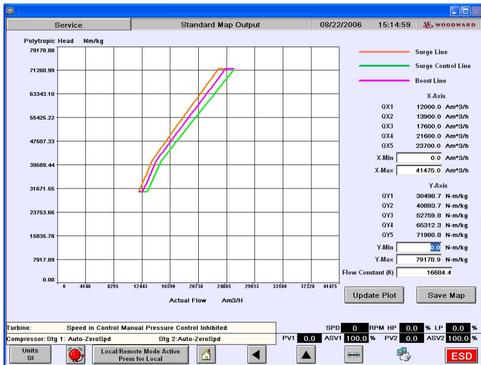
Figure 4-16. Standard Map Output Screen
