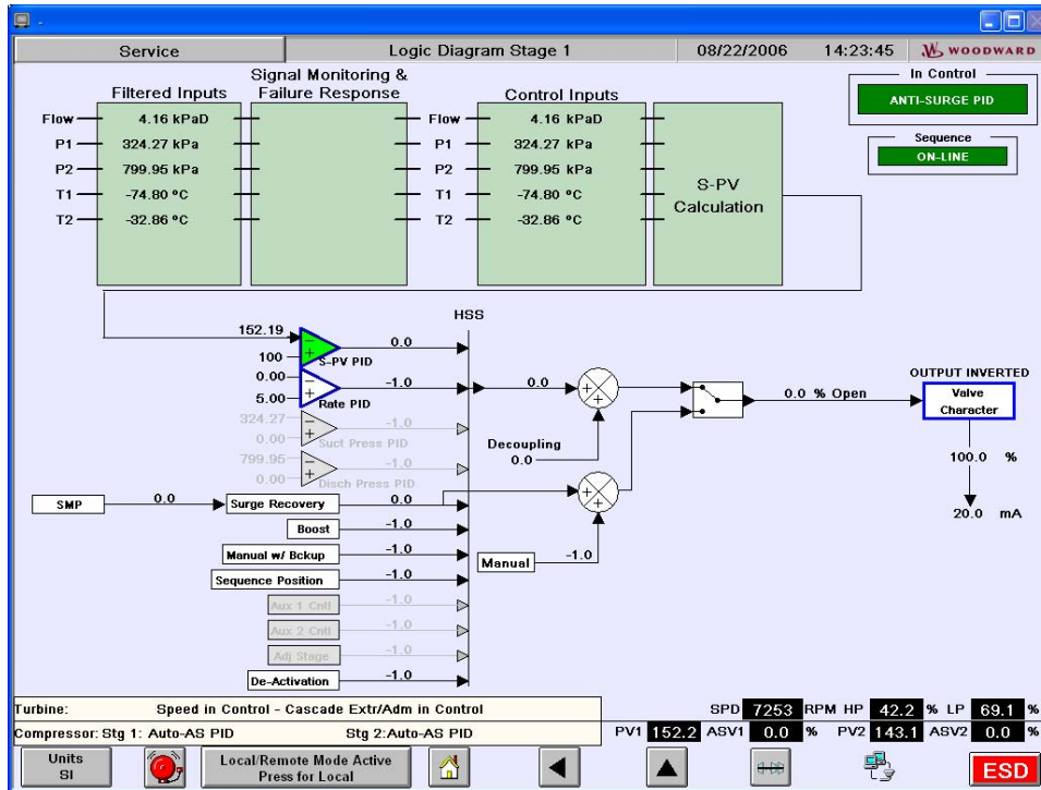
Figure 5-4. Compressor Logic Diagram Screen
