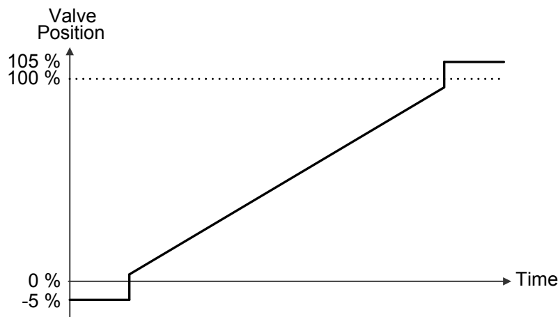
Figure 2-28. Valve Overstroke
