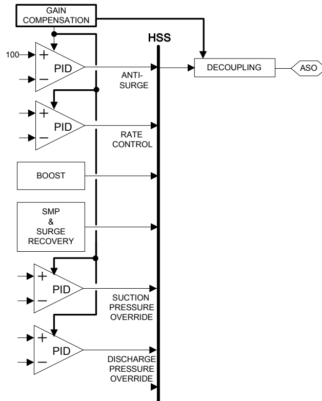
Figure 2-20. Automatic Gain Compensation
