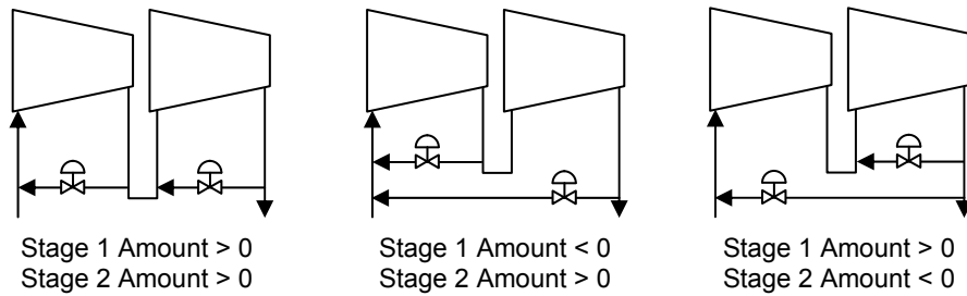
Figure 2-22. Effect of Valve Layout on Adjacent Stage Decoupling Amounts
