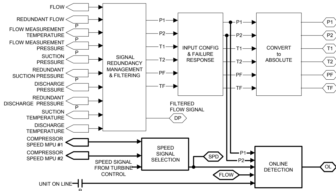
Figure 2-12. On-Line Detection
