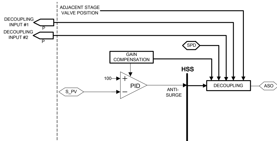
Figure 2-21. Anti-Surge Decoupling
