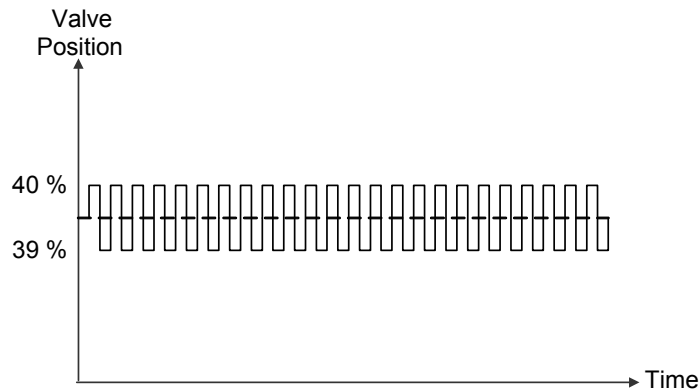
Figure 2-29. Valve Dither
