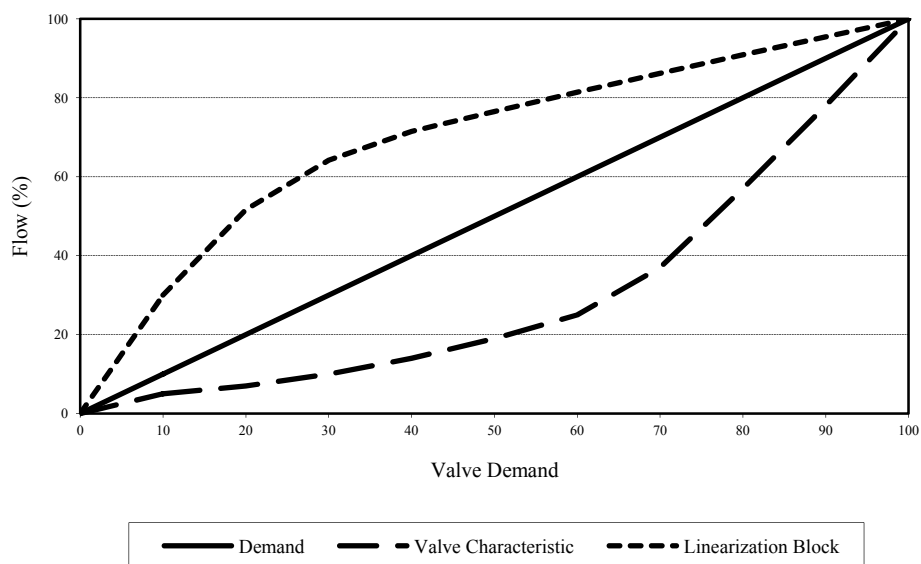
Figure 2-30. Valve Characterization
