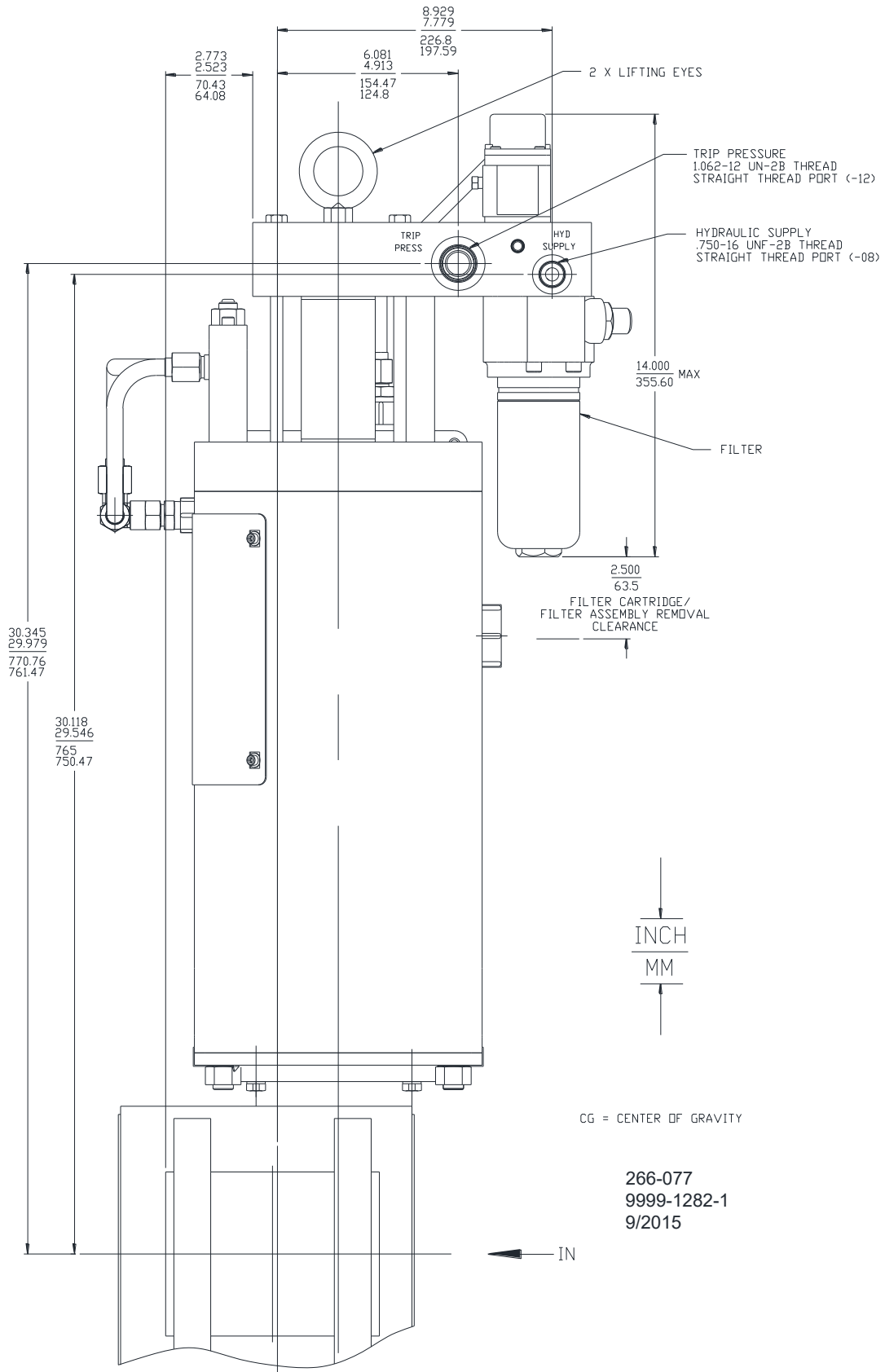
Figure 1-5d. Gas Stop/Ratio Valve Outline Drawing (3-inch High Pressure Trip (HPT))
