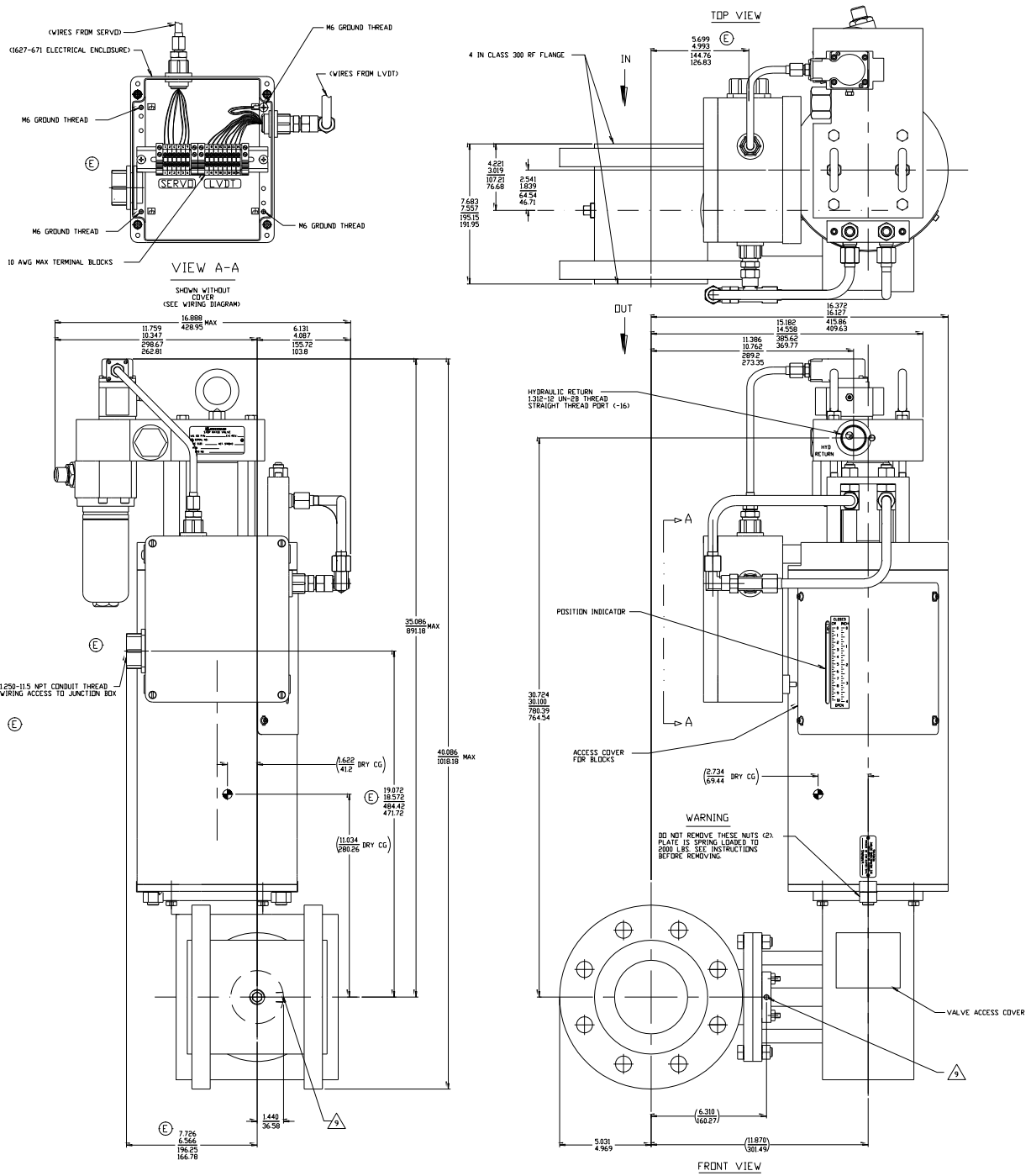
Figure 1-6a. Gas Stop/Ratio Valve Outline Drawing (4-inch)
