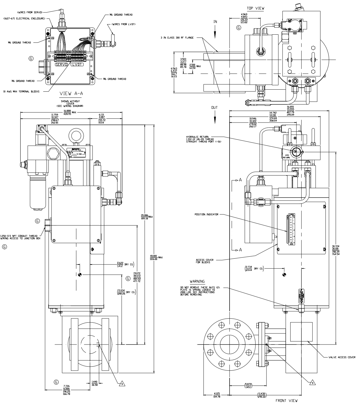
Figure 1-5a. Gas Stop/Ratio Valve Outline Drawing (3-inch) Low Pressure Trip (LPT)
