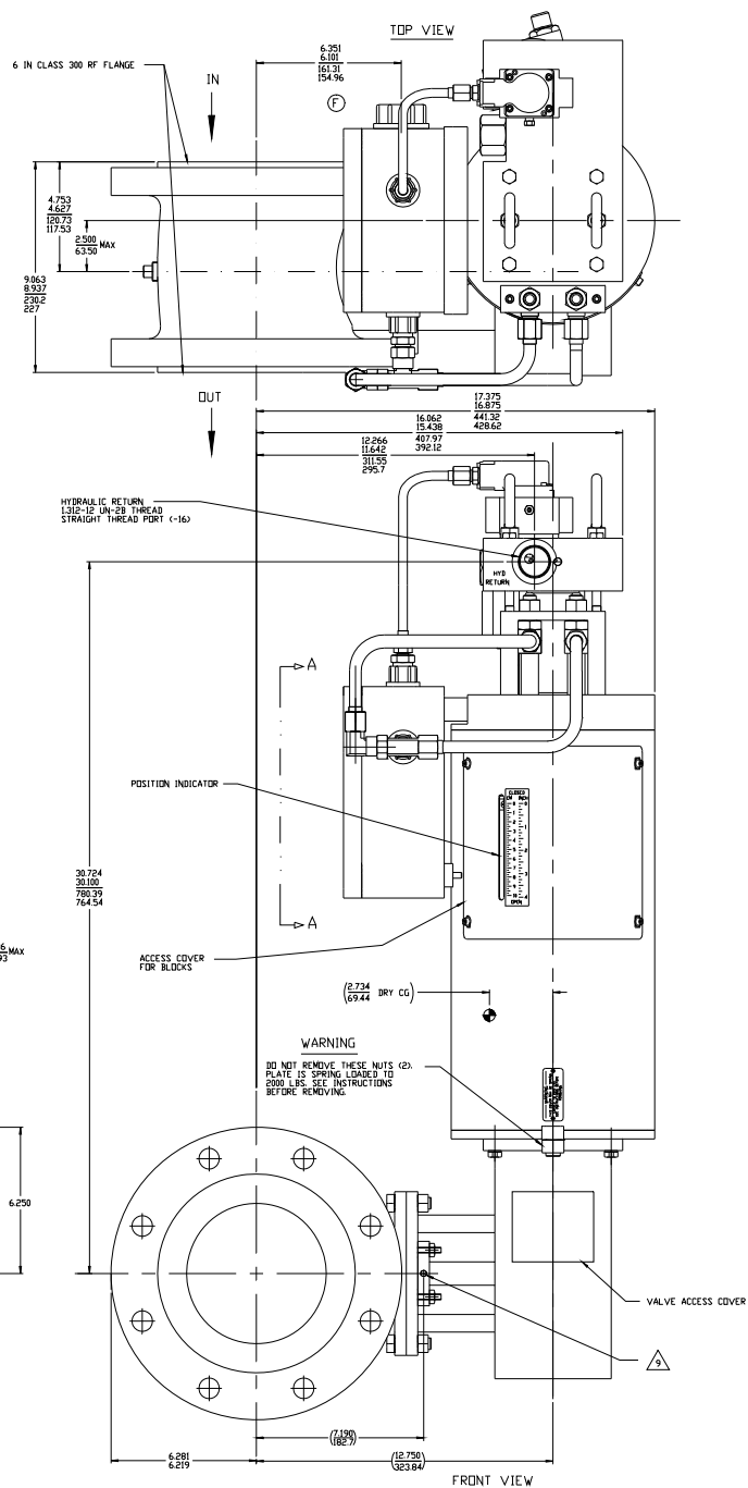
Figure 1-7a. Gas Stop/Ratio Valve Outline Drawing (6-inch, except SS-260)
