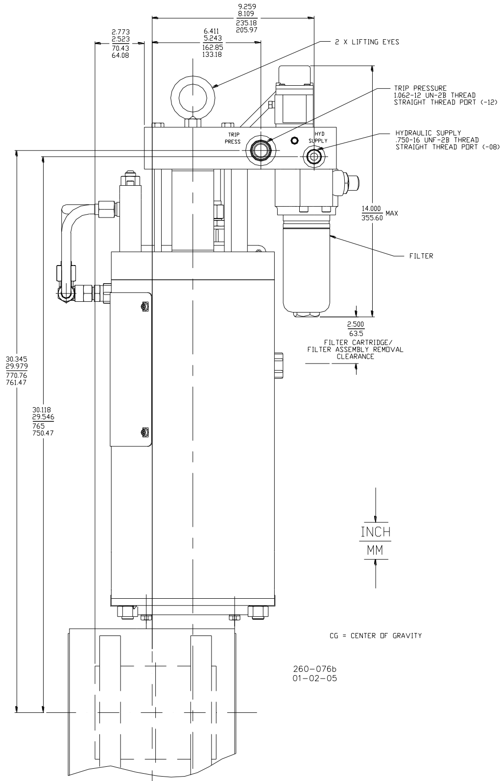
Figure 1-5b. Gas Stop/Ratio Valve Outline Drawing (3-inch) Low Pressure Trip (LPT)
