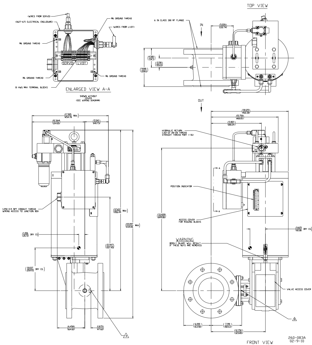
Figure 1-8a. Gas Stop/Ratio Valve Outline Drawing (6-inch, SS-260)
