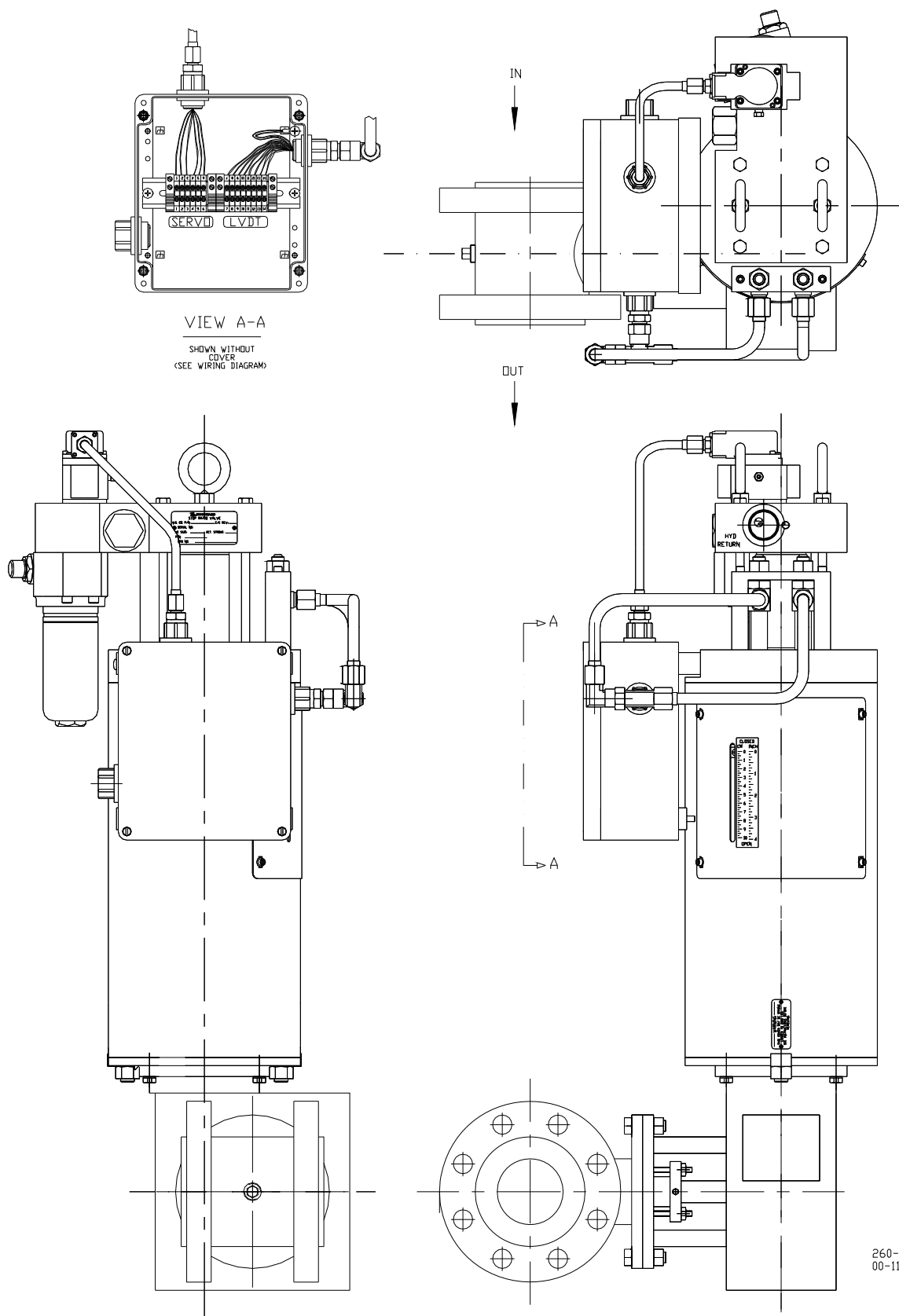
Figure 1-1. Gas Stop/Ratio Valve (typical; 3-inch shown)
