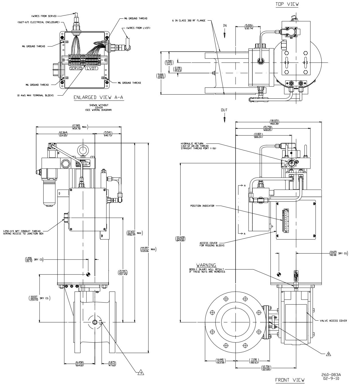
Figure 1-8a. Gas Stop/Ratio Valve Outline Drawing (6-inch, SS-260)
