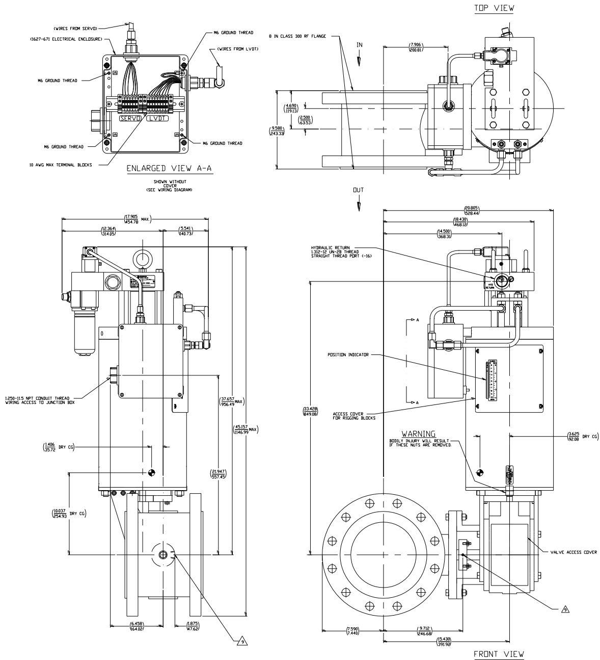
Figure 1-10a. Gas Stop/Ratio Valve Outline Drawing (8-inch, with 2 LVDTs)
