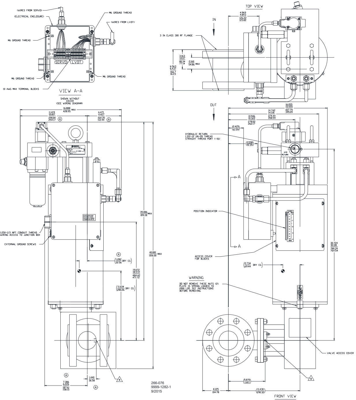
Figure 1-5c. Gas Stop/Ratio Valve Outline Drawing (3-inch) High Pressure Trip (HPT)
