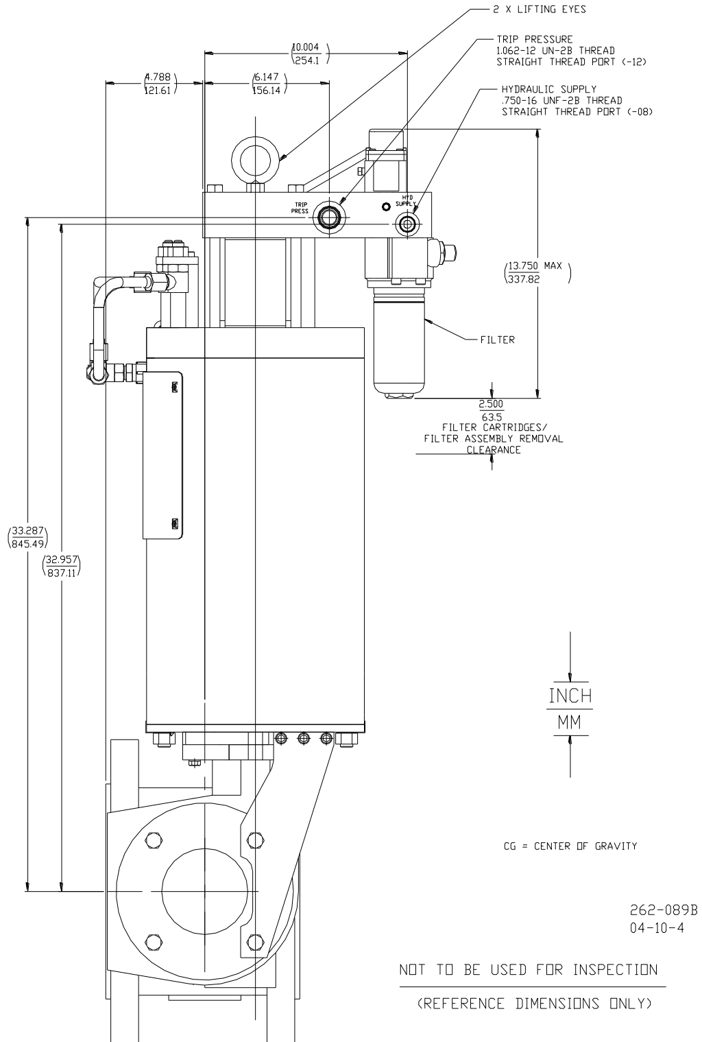
Figure 1-11b. Gas Stop/Ratio Valve Outline Drawing (8-inch, with 3 LVDTs)
