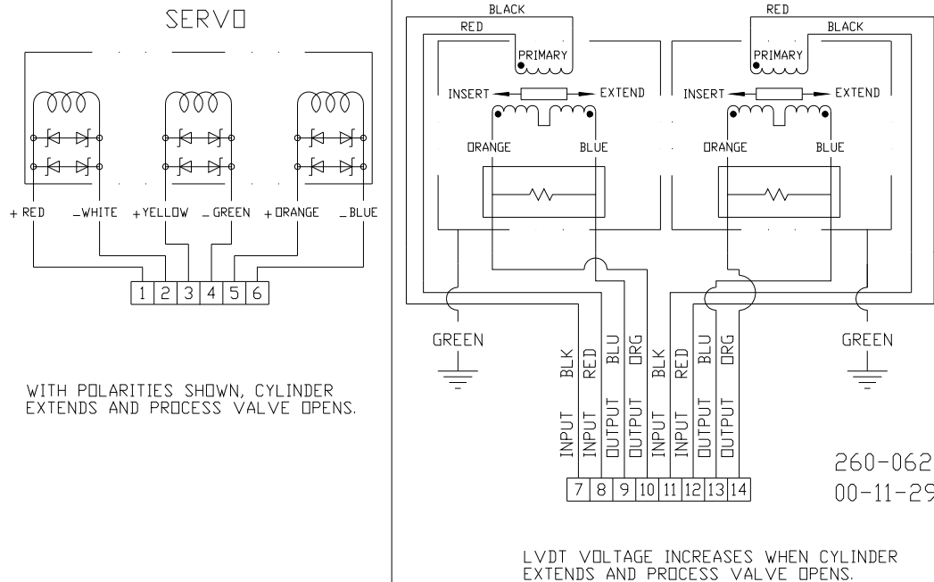
Figure 1-3a. Electrical Schematic and Wiring Diagram (Dual LVDT)
