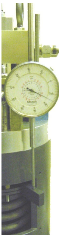
Figure 5-3. Stroke Measurement Attachment Bar
