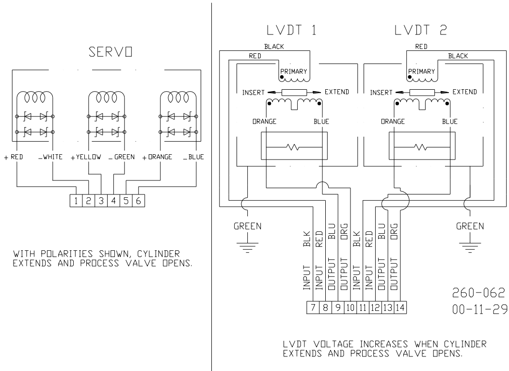
Figure 1-3a. Electrical Schematic and Wiring Diagram (Dual LVDT)
