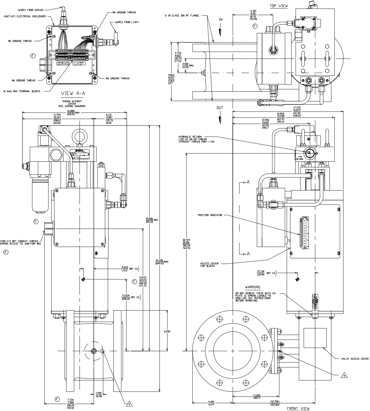
Figure 1-7a. Gas Stop/Ratio Valve Outline Drawing (6-inch, except SS-260)
