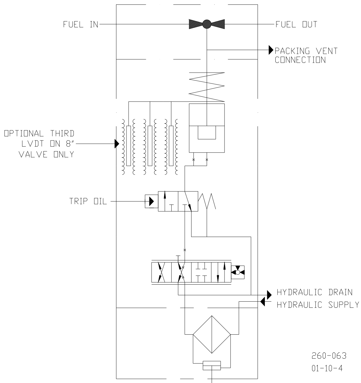
Figure 1-2. Single Acting Hydraulic Schematic
