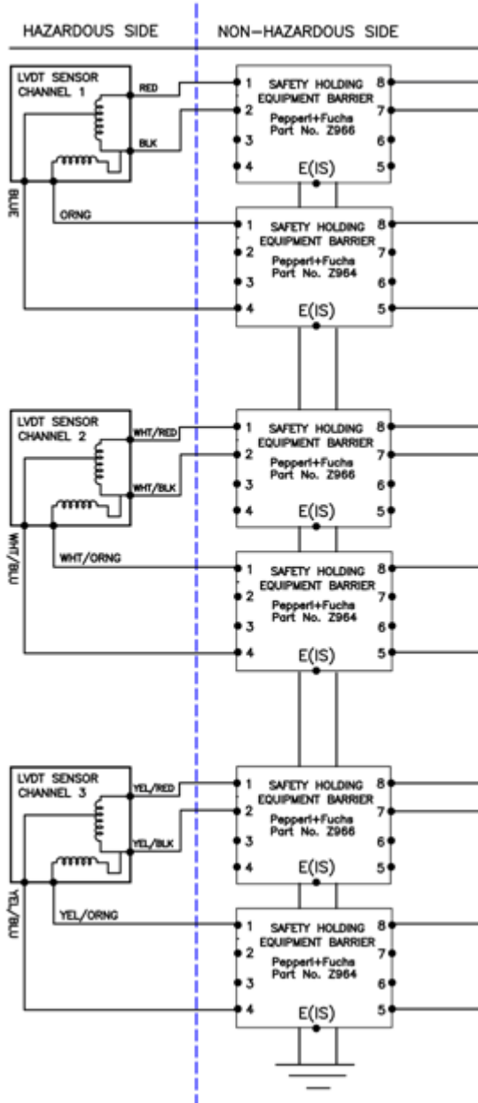
Figure 1-4a. LVDT Barrier Wiring Diagram (TIIS requirement, Japan) [This figure applies to TIIS requirement for Japan only.]
