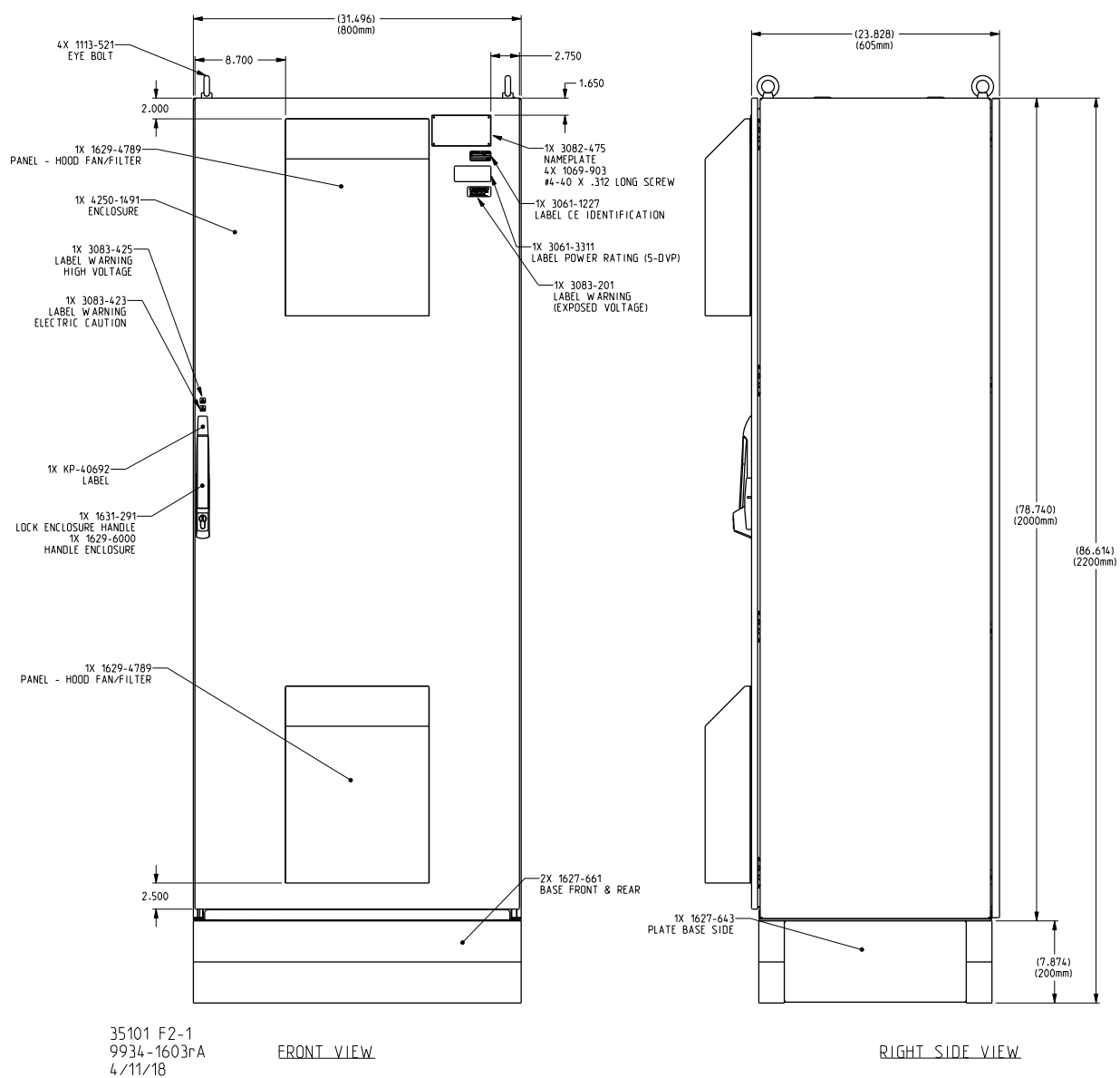
Figure 2-1. Outline Drawing
