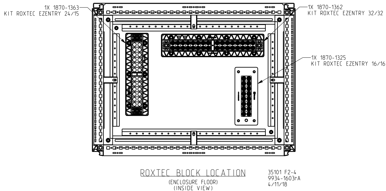
Figure 2-4. Position of Roxtec Blocks
