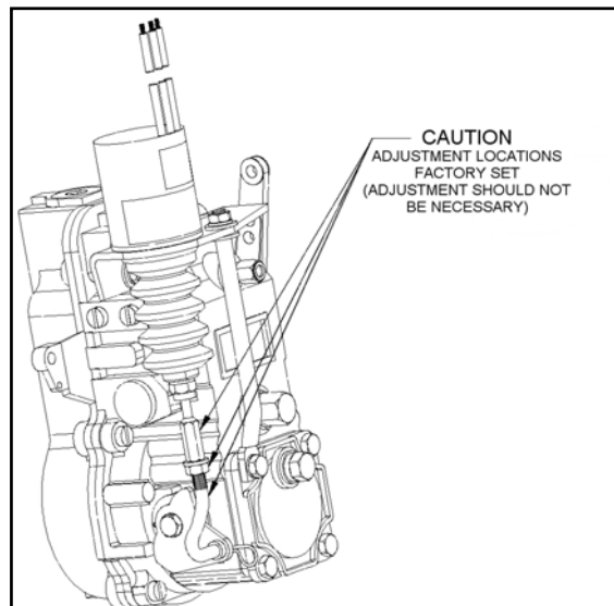
Figure 3. Parts View
