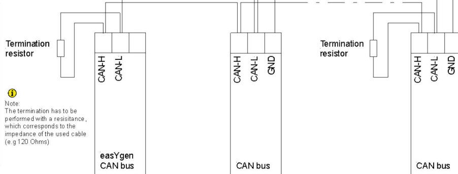
Figure 5-34: Interfaces - CAN bus - termination
