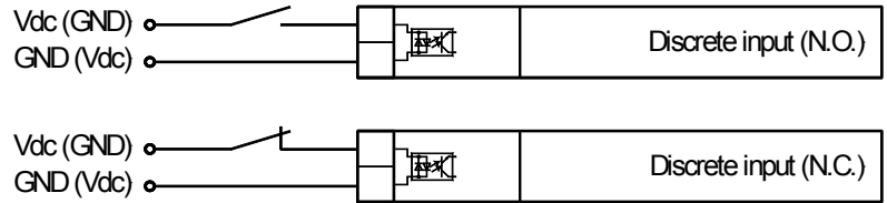
Figure 5-27: Discrete inputs - alarm/control inputs - operation logic
