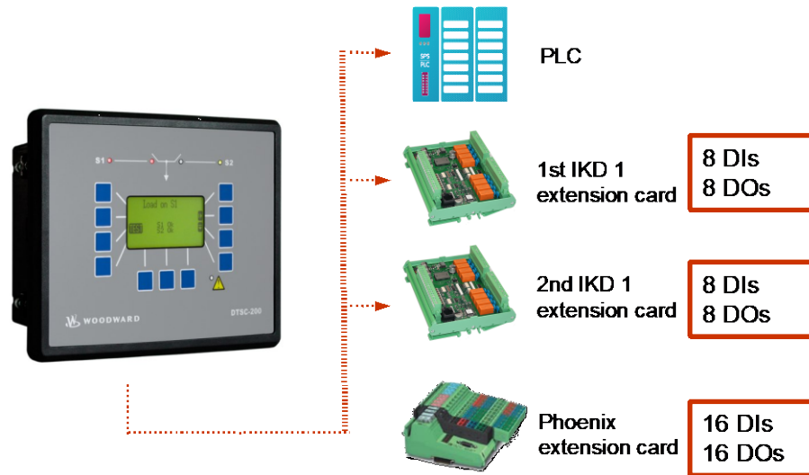
Figure 4-3: CANopen interface - external devices
