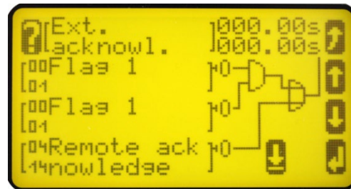
Figure 4-7: Display screen - Ext. acknowledge
