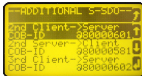
Figure 4-12: Display screen - configure Server SDOs
