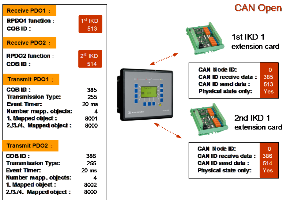
Figure 4-5: CANopen interface - expansion with two IKD 1
