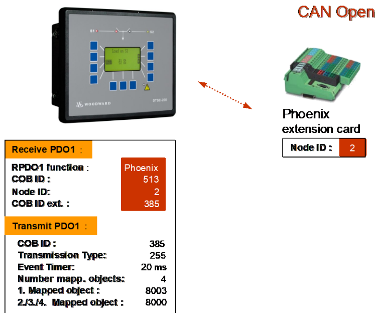
Figure 4-6: CANOpen interface - expansion with Phoenix terminal
