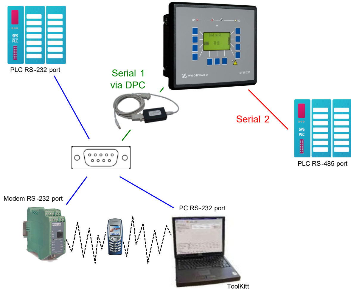
Figure3-1: Serial interface - overview
