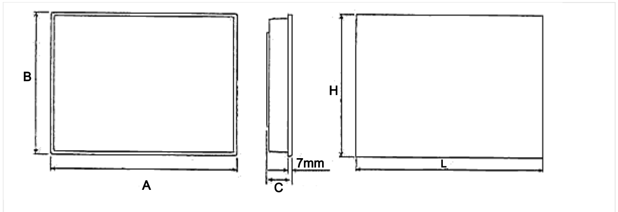
Fig. 8: Dimension and cut out
