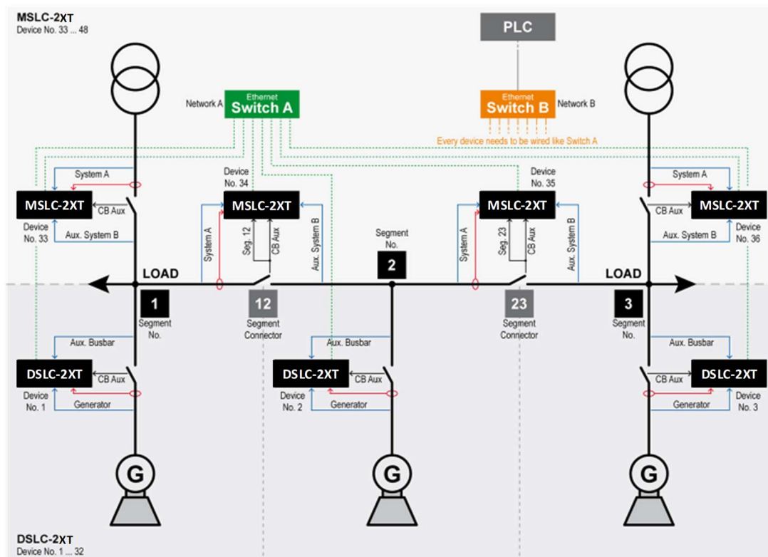
Configuration of a typical application using DSLC-2XT and MSLC-2XT devices in combination
