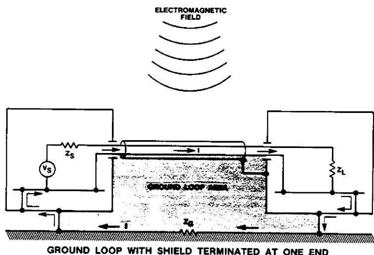
Figure 9. Ground Loop with Shield Terminated at One End—No Shielding of Magnetic Field Occurs
