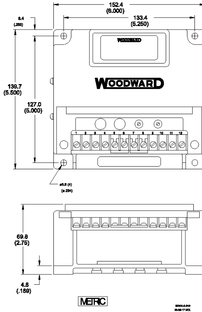
Outline Drawing (Do not use for construction)
