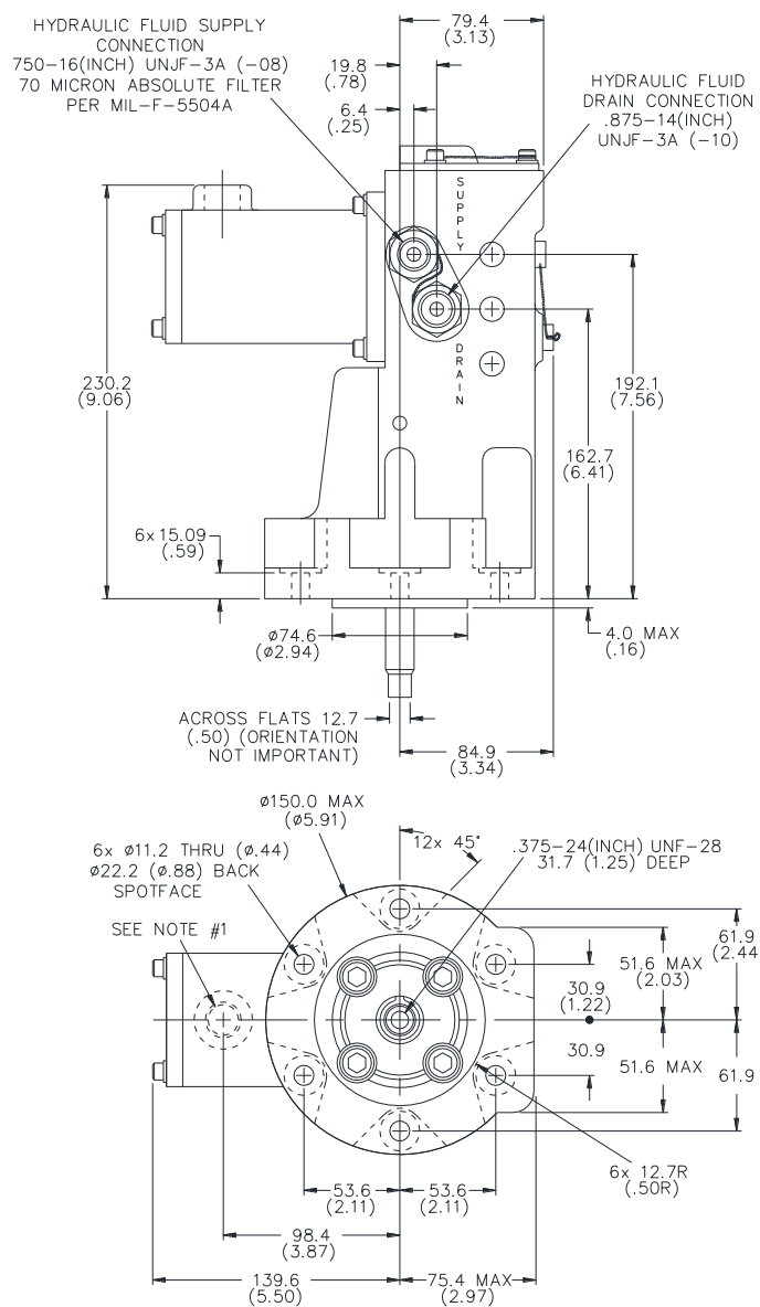
Figure 2-1a. TM-25LP/TM-200LP Actuator
