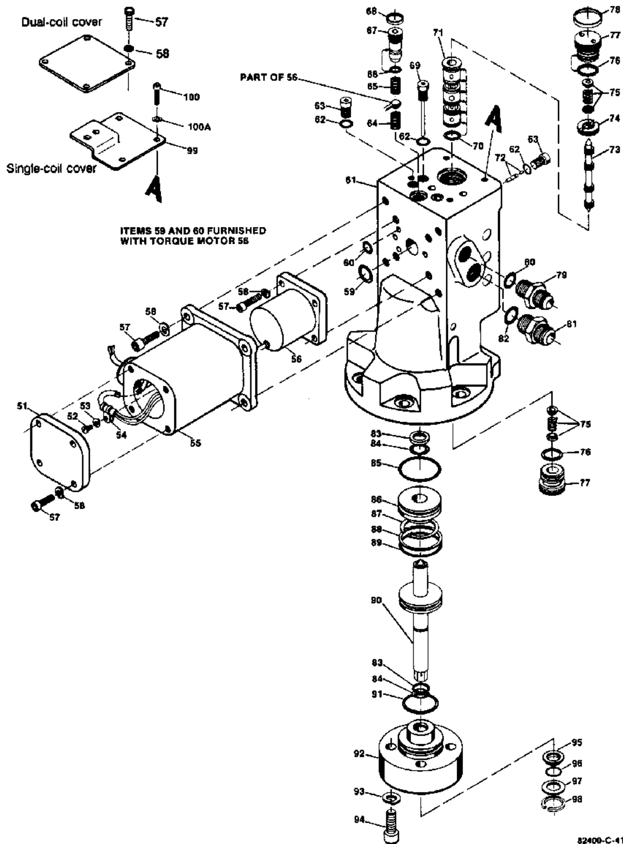
Figure 6-1. TM-200LP Exploded View
