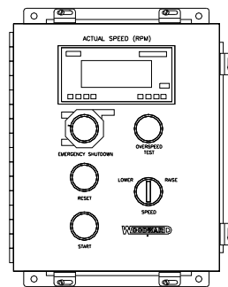
OPTIONAL ROLLING RESTART STATION
