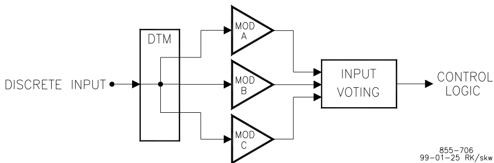
Figure 2-4. Fault Tolerant Discrete Input
