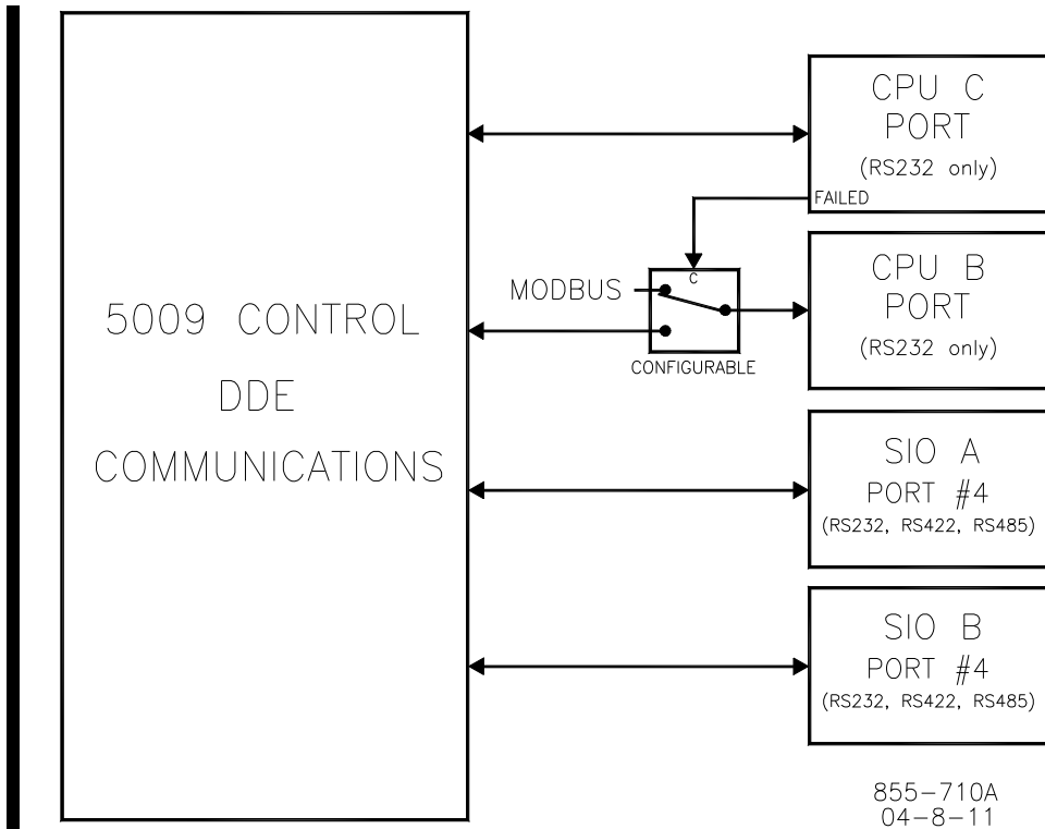
Figure 2-9. Fault Tolerant DDE Communication Ports
