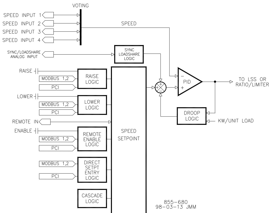
Figure 5-6. Speed Control Functional Diagram
