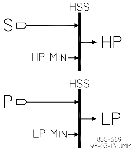
Figure 5-15. Decoupled HP&amp;LP Mode
