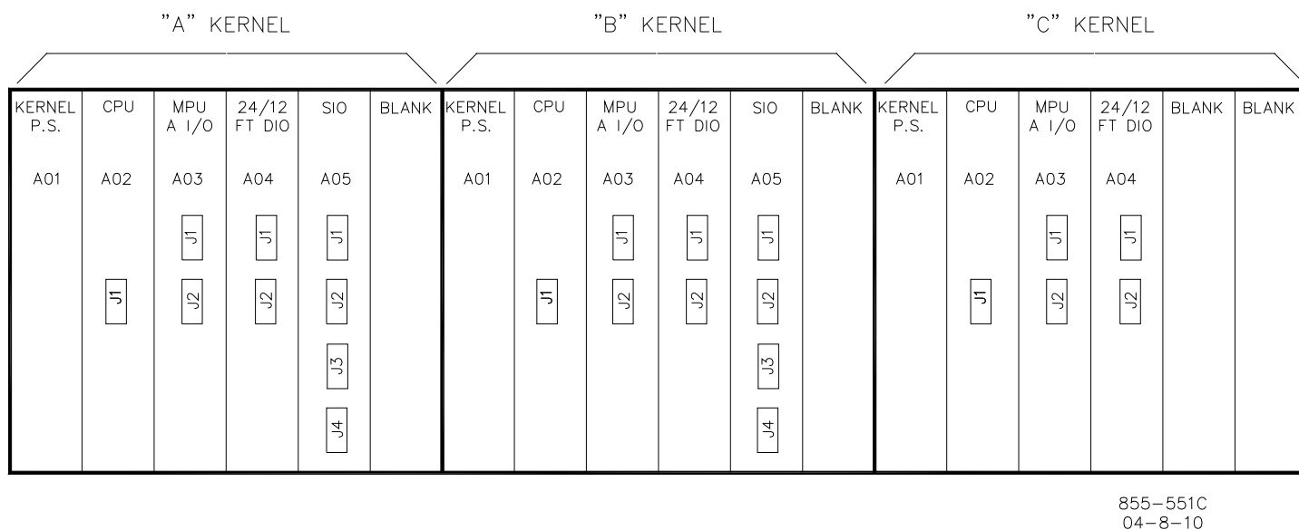
Figure 2-1. System Module Diagram
