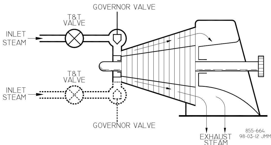
Figure 3-1. Typical Single Valve or Split Range Valve Steam Turbine
