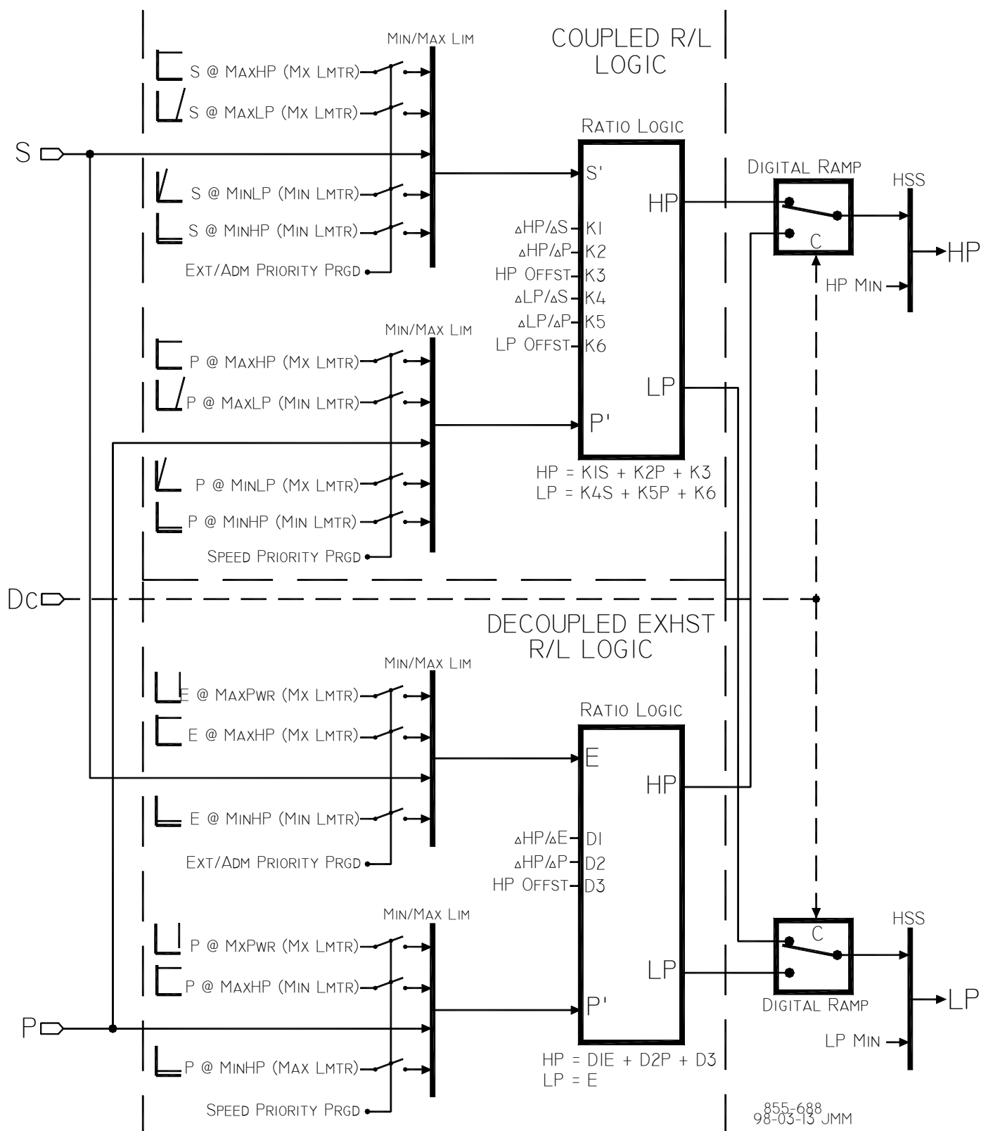
Figure 5-14. Decoupled Exhaust (LP) Mode
