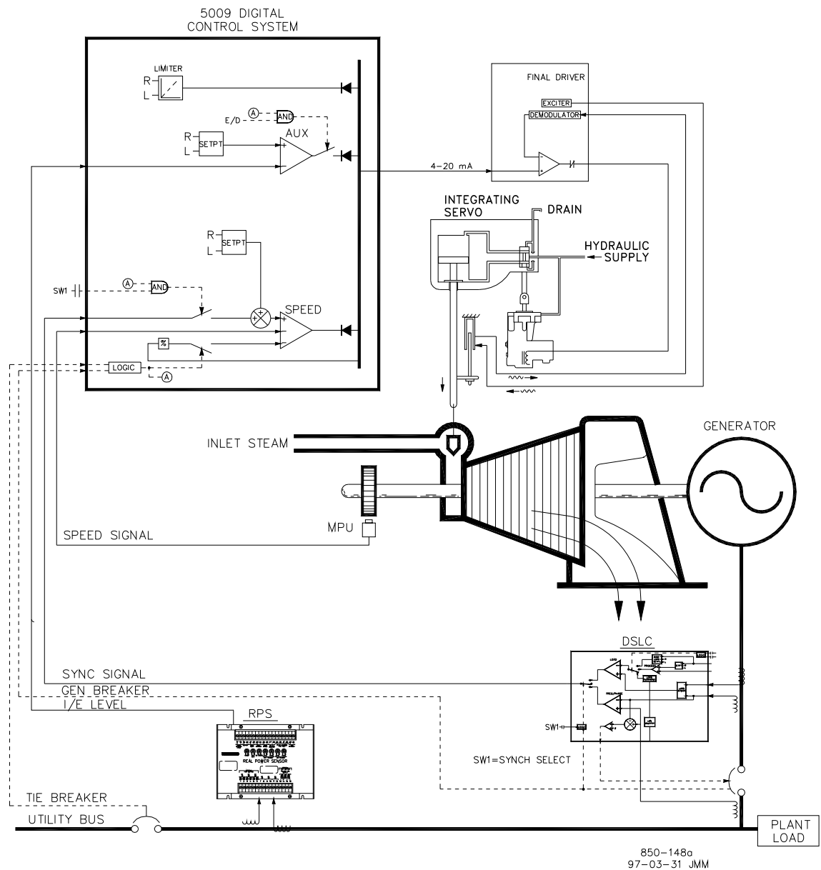
Figure 4-4. Plant Import/Export Control with DRFD Servo Interface
