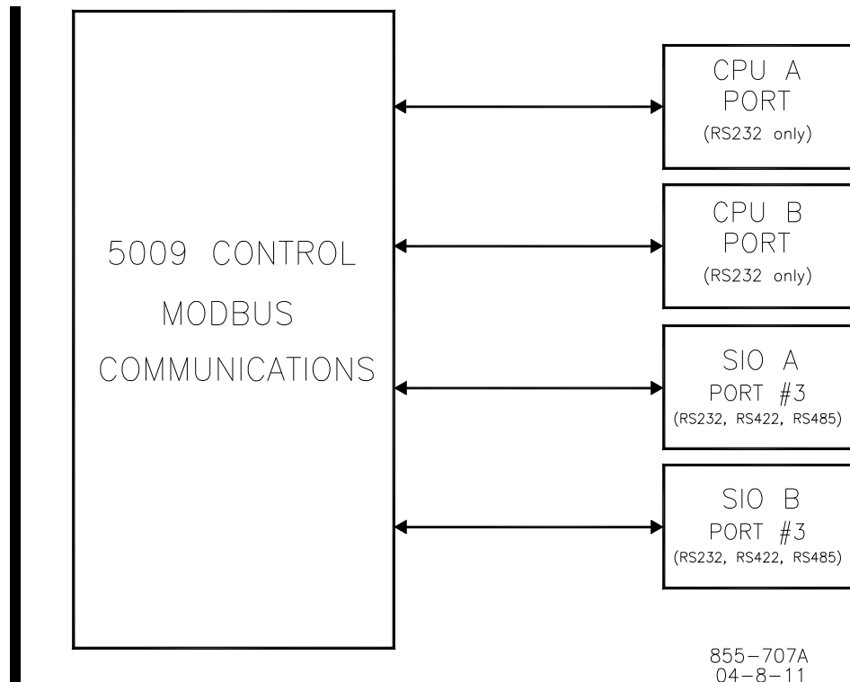
Figure 2-10. Fault Tolerant Modbus Communication Ports
