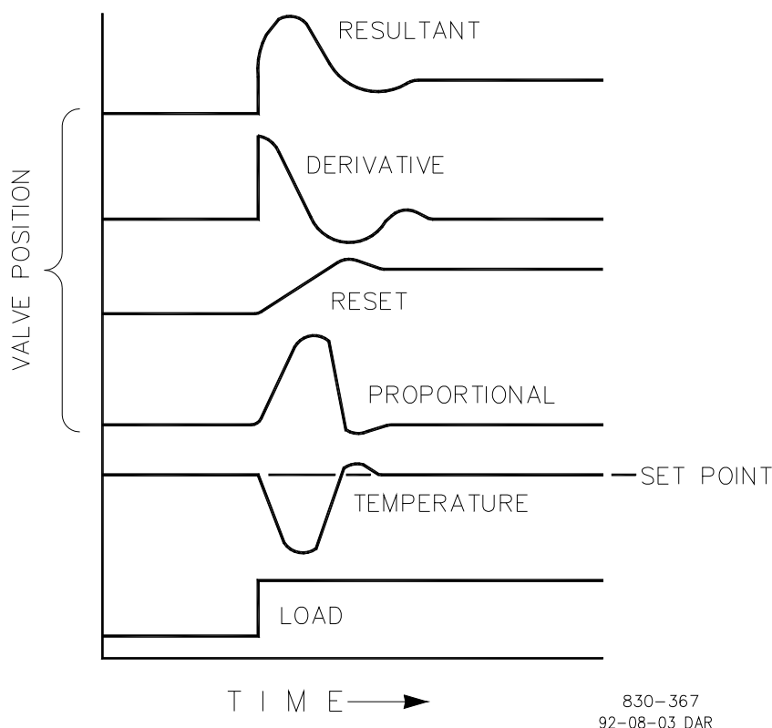
Figure 6-7. Closed Loop Proportional, Integral and Derivative Action
