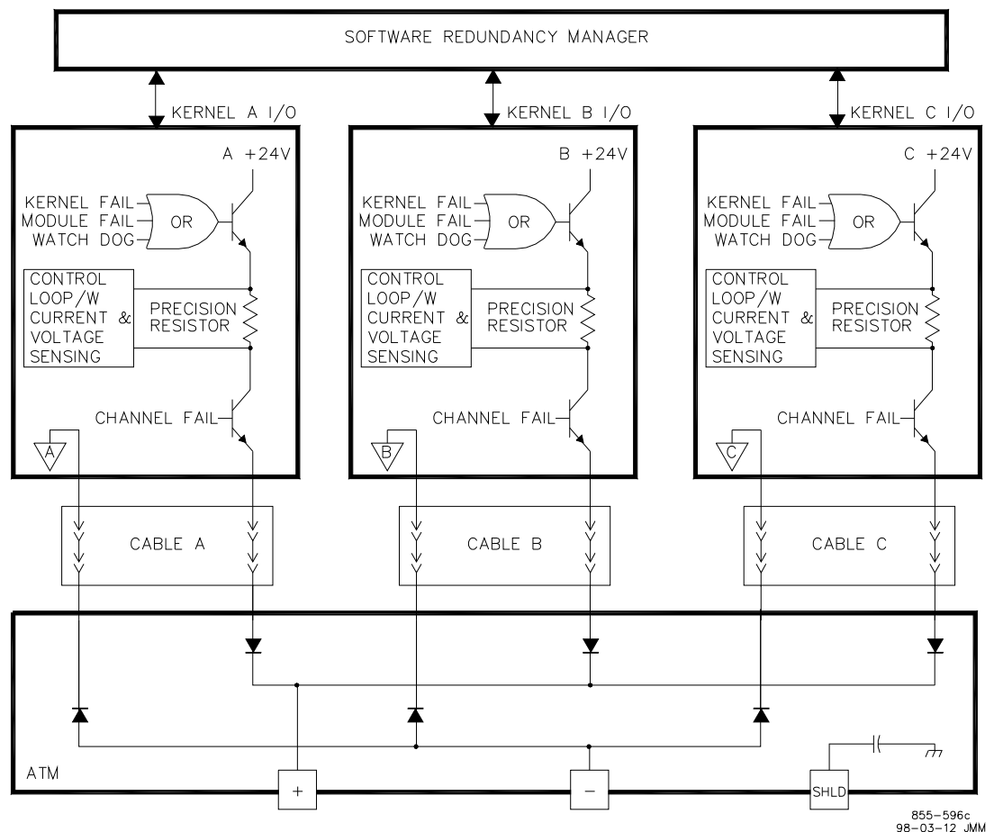
Figure 2-5. Fault Tolerant Analog Output
