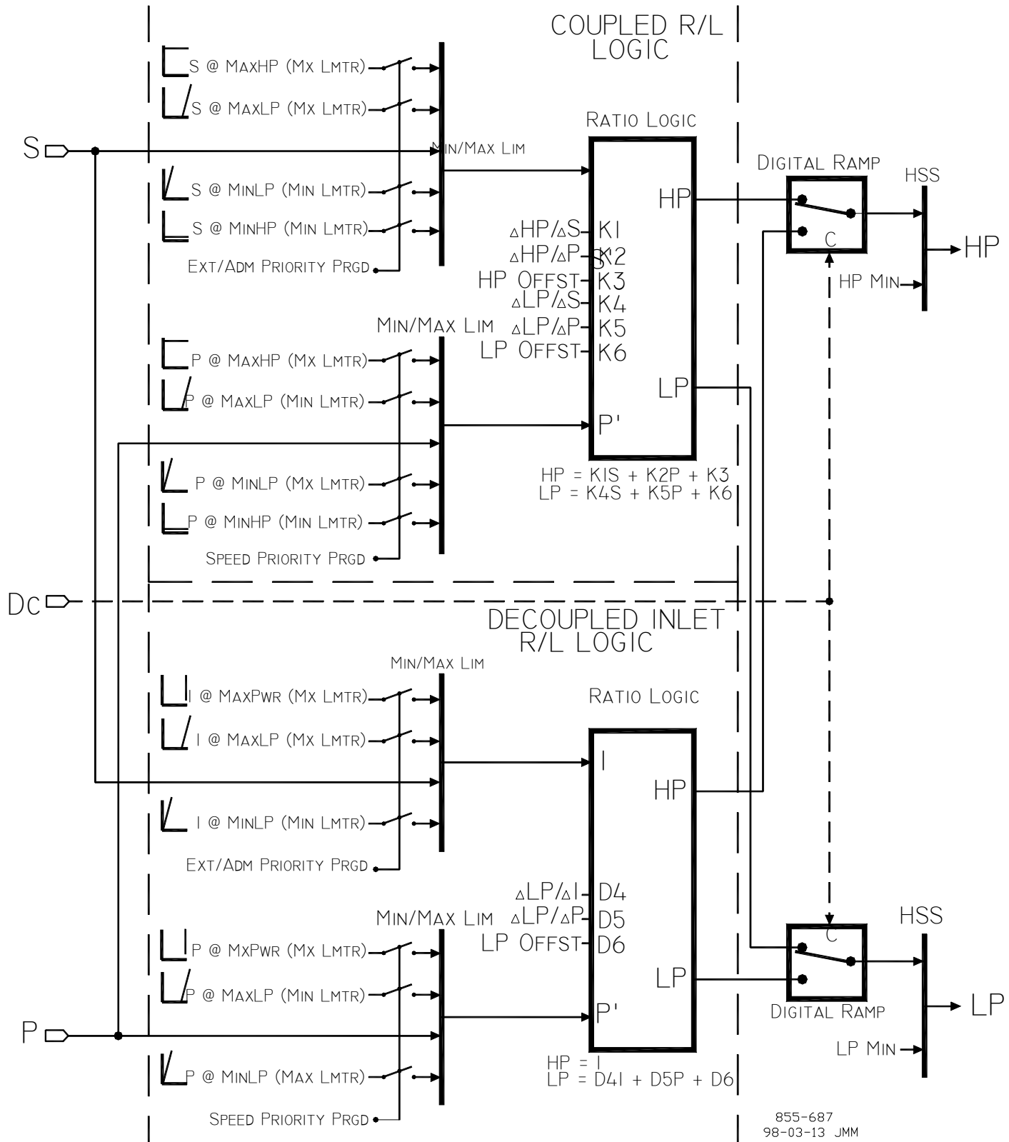
Figure 5-13. Decoupled Inlet (HP) Mode
