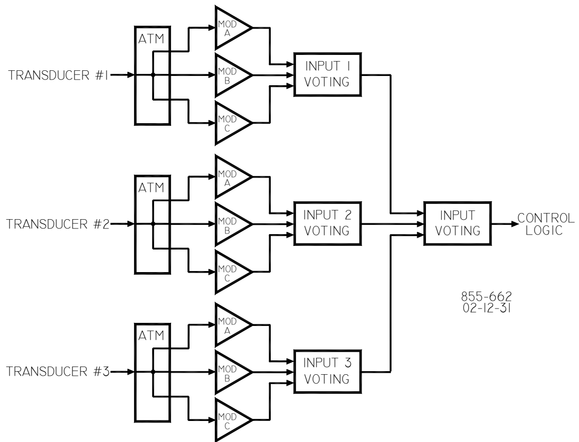
Figure 2-3. Fault Tolerant Analog Input
