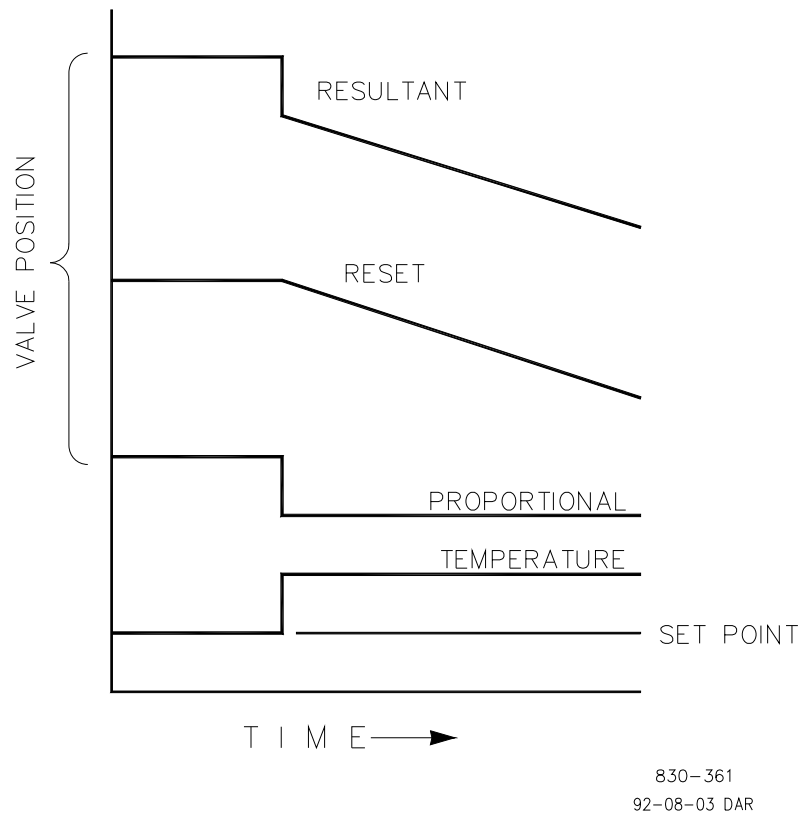
Figure 6-2. Open Loop Proportional and Integral Response
