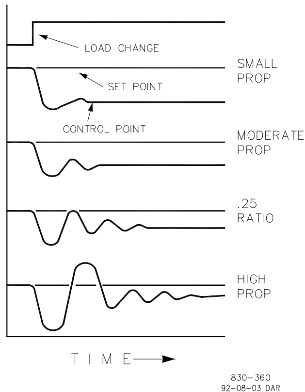
Figure 6-1. Proportional Gain Setting Effects
