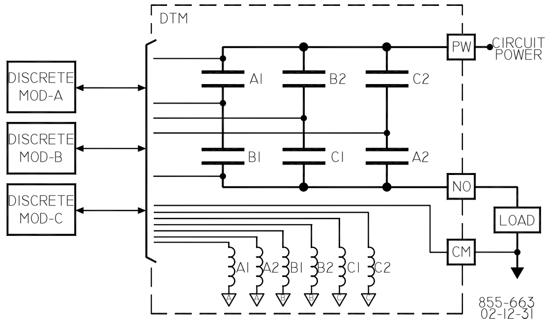
Figure 2-8. Fault Tolerant Discrete Output
