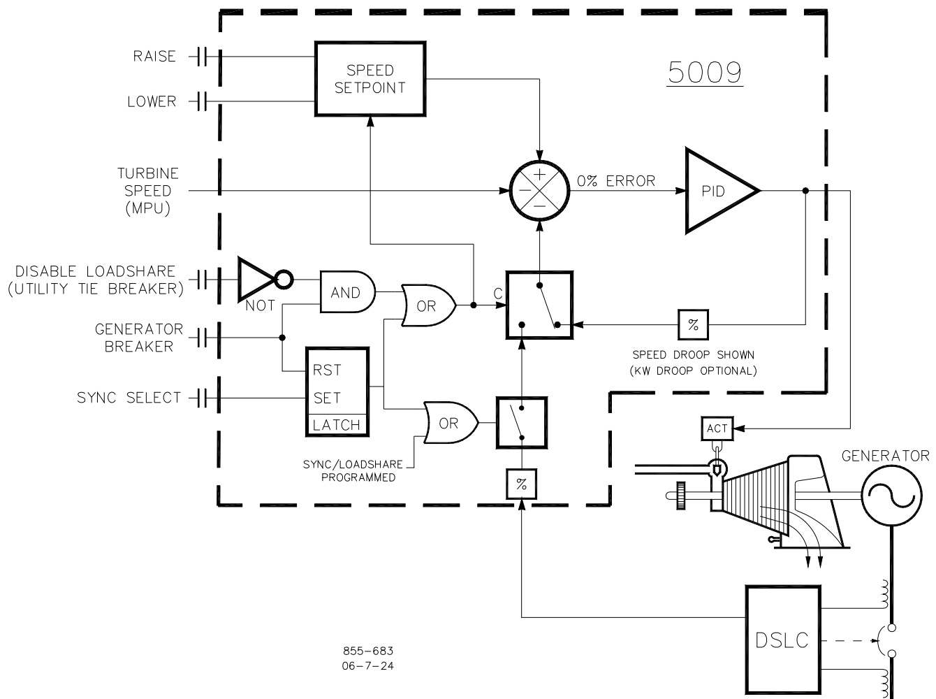
Figure 5-10. Loadsharing Logic
