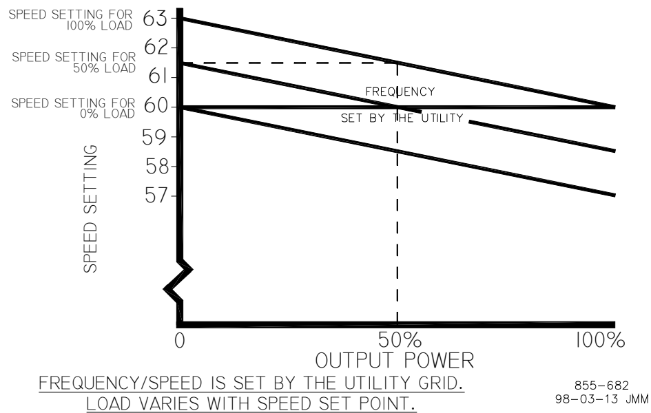
Figure 5-8. Frequency and Unit Load Relationship
