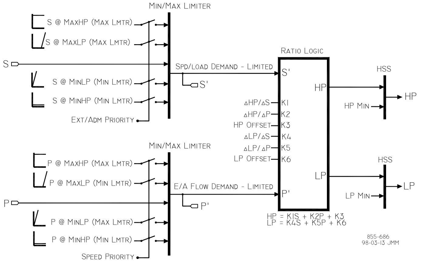
Figure 5-12. Coupled HP &amp; LP Mode
