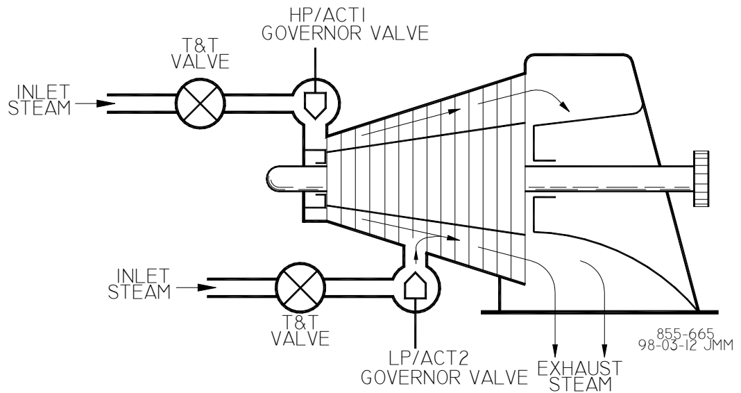
Figure 3-2. Split Range or Admission Type of Turbine Configuration (depending on the parameters being controlled)
