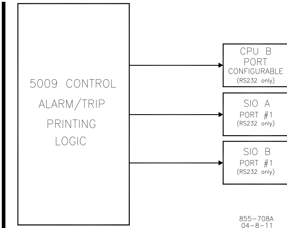
Figure 2-11. Fault Tolerant Modbus Communication Ports
