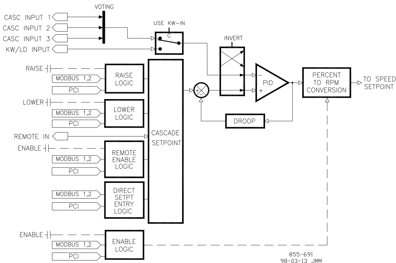
Figure 5-18. Cascade Functional Diagram
