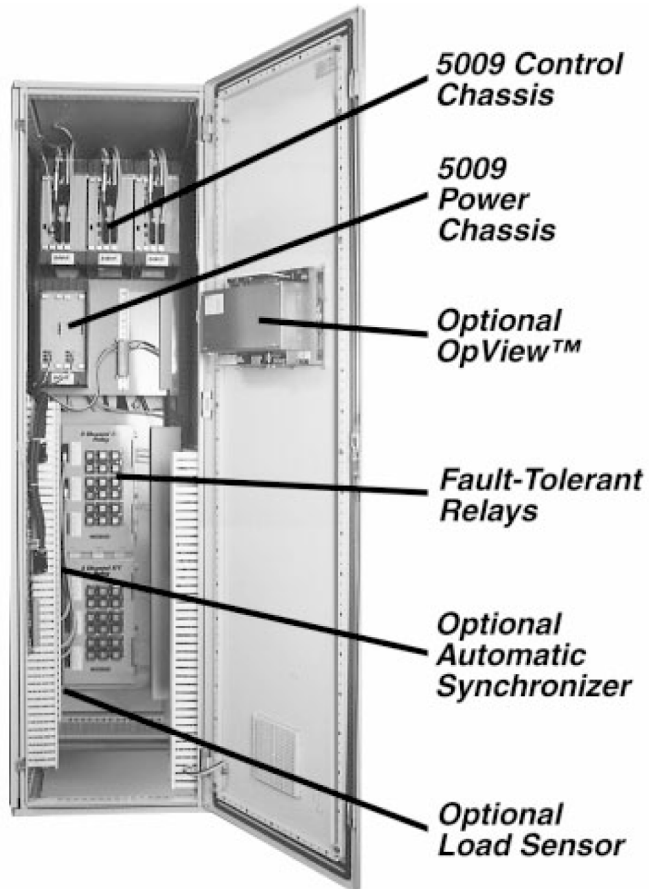
Figure 1-1. Cabinet System Overview
