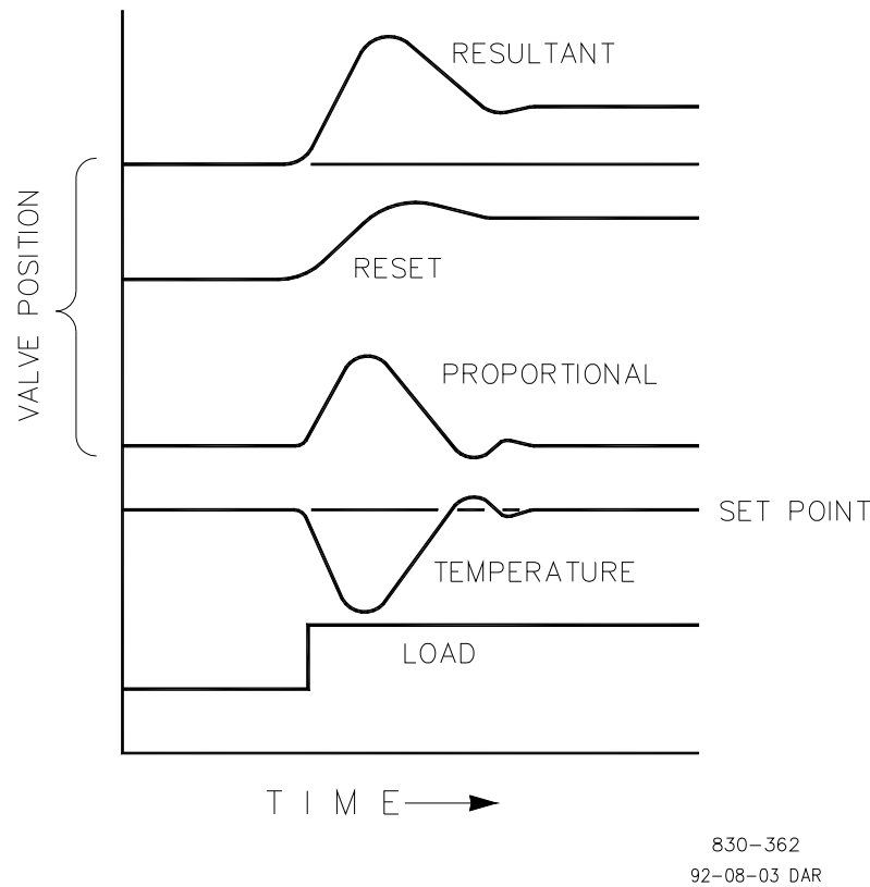
Figure 6-3. Closed Loop Proportional and Integral Response
