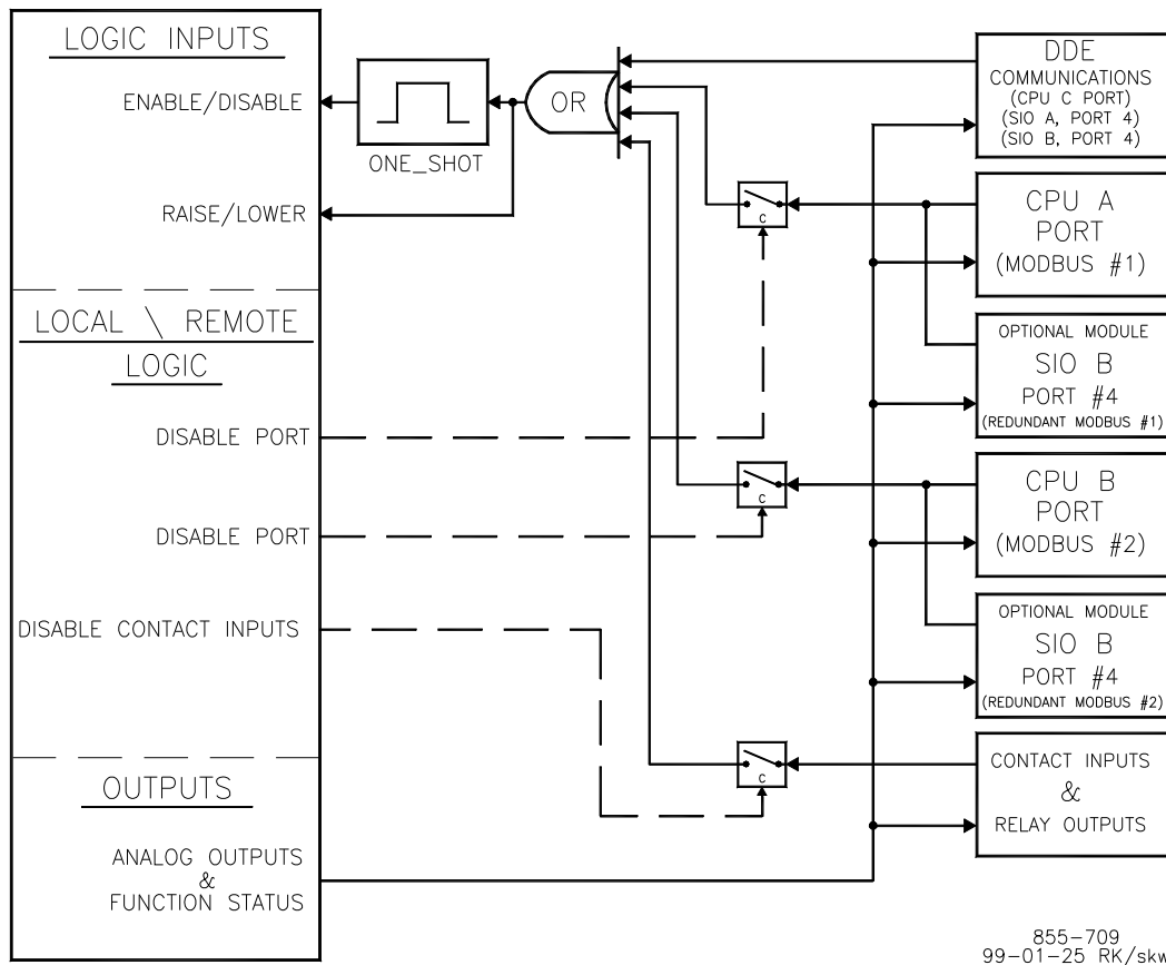
Figure 2-12. Interface/Communications Logic
