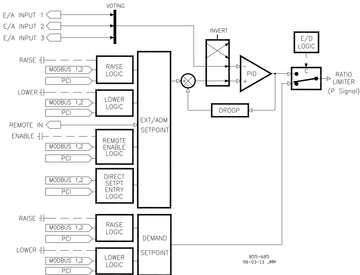
Figure 5-11. Ext/Adm Control Diagram
