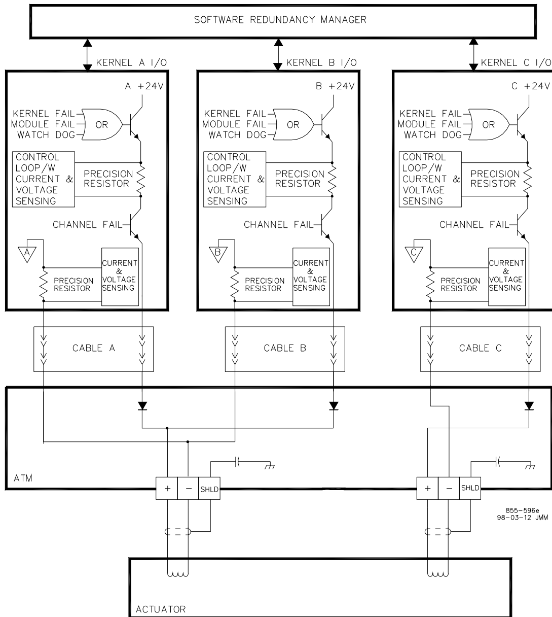
Figure 2-7. Fault Tolerant Dual Coil Actuator Output
