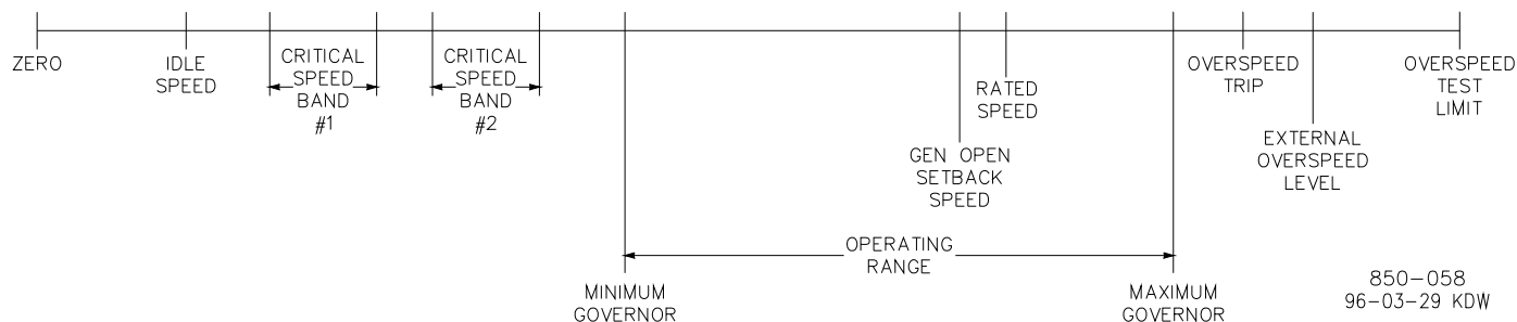
Figure 5-9. Speed Relationships
