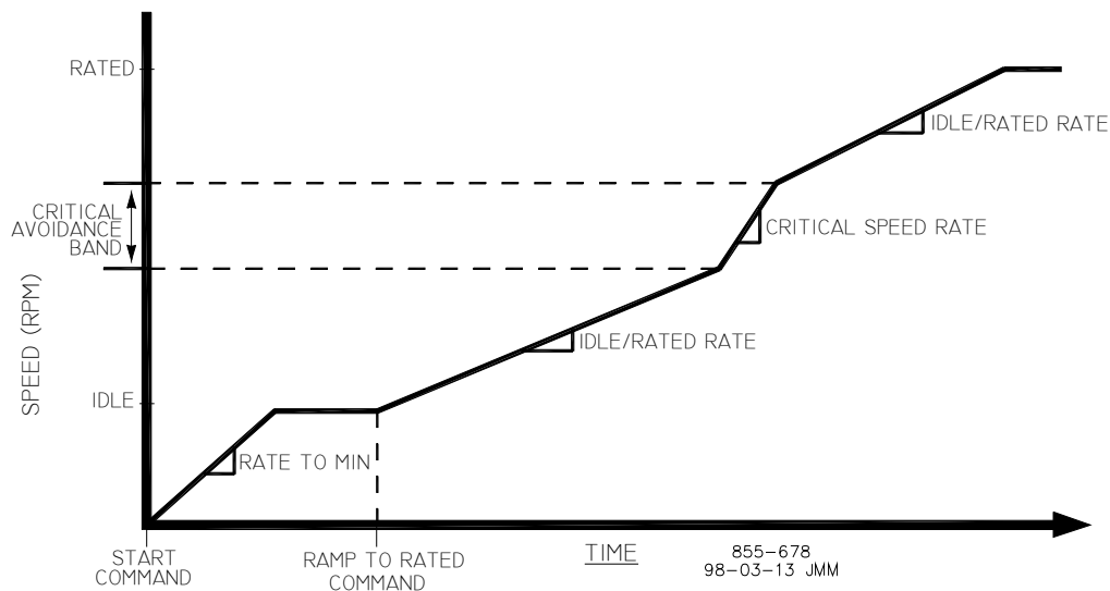
Figure 5-4. Idle / Rated Start
