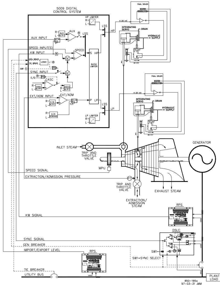
Figure 4-5. Plant Import/Export Control with DRFD Servo Interface
