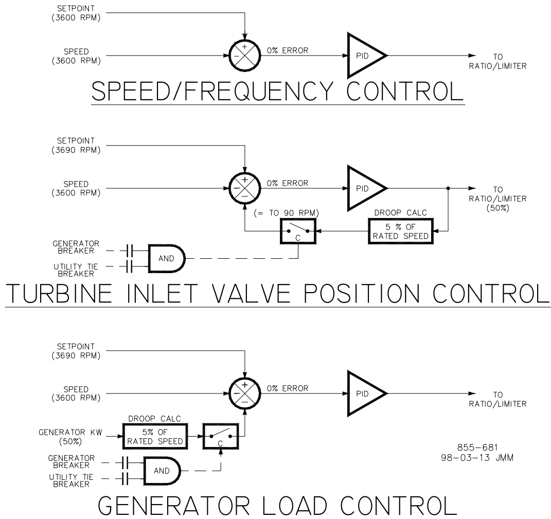
Figure 5-7. Speed PID Control Modes
