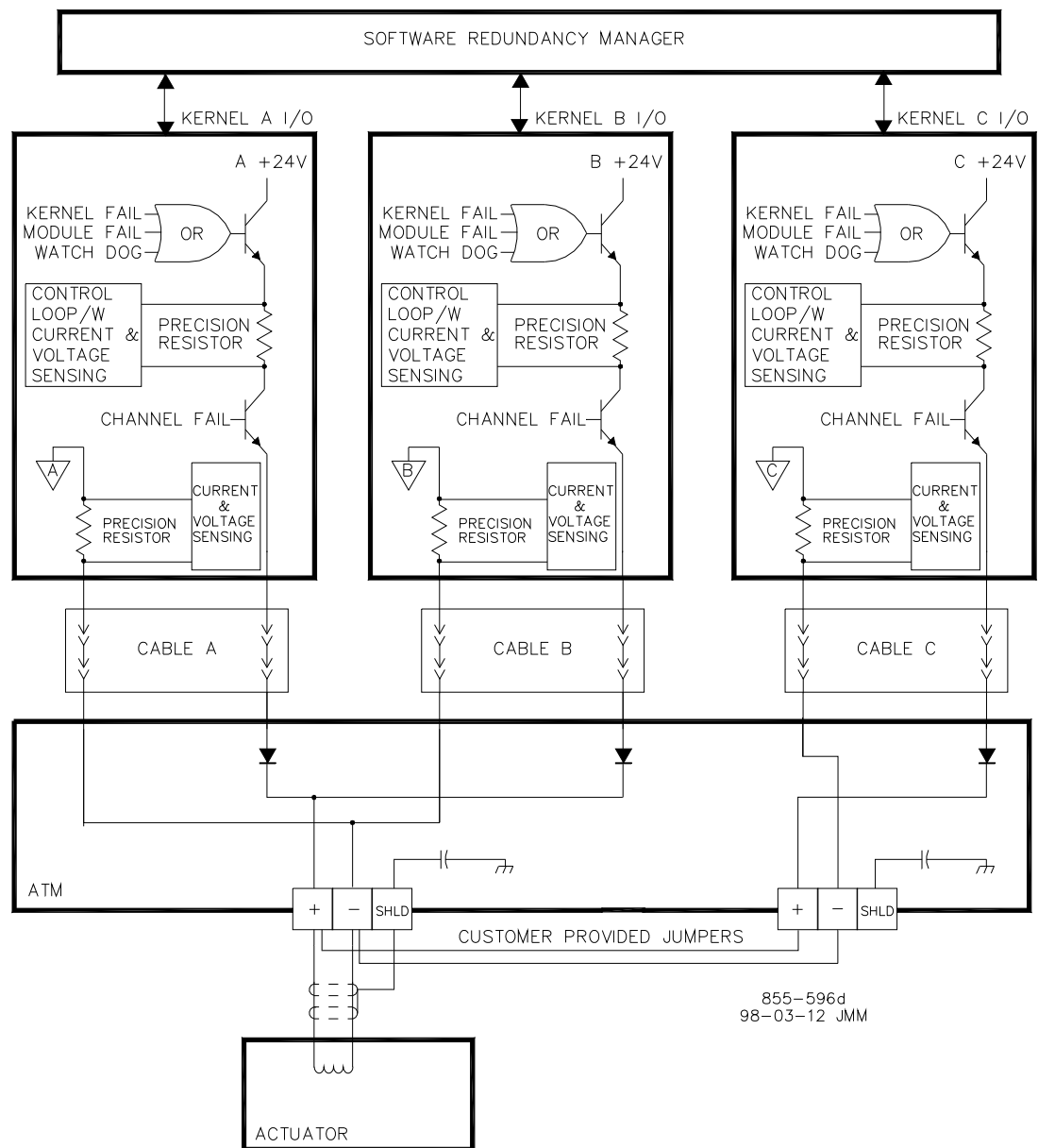
Figure 2-6. Fault Tolerant Single Coil Actuator Output
