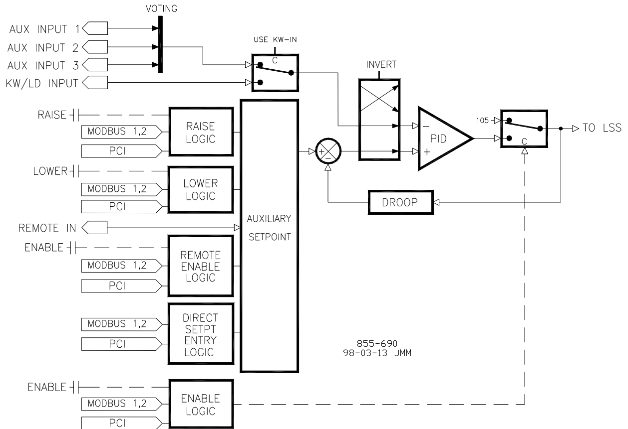
Figure 5-17. Auxiliary Control Overview
