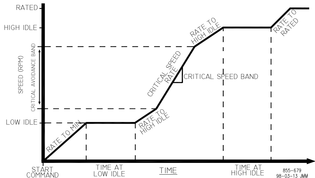
Figure 5-5. Automatic Start Sequence
