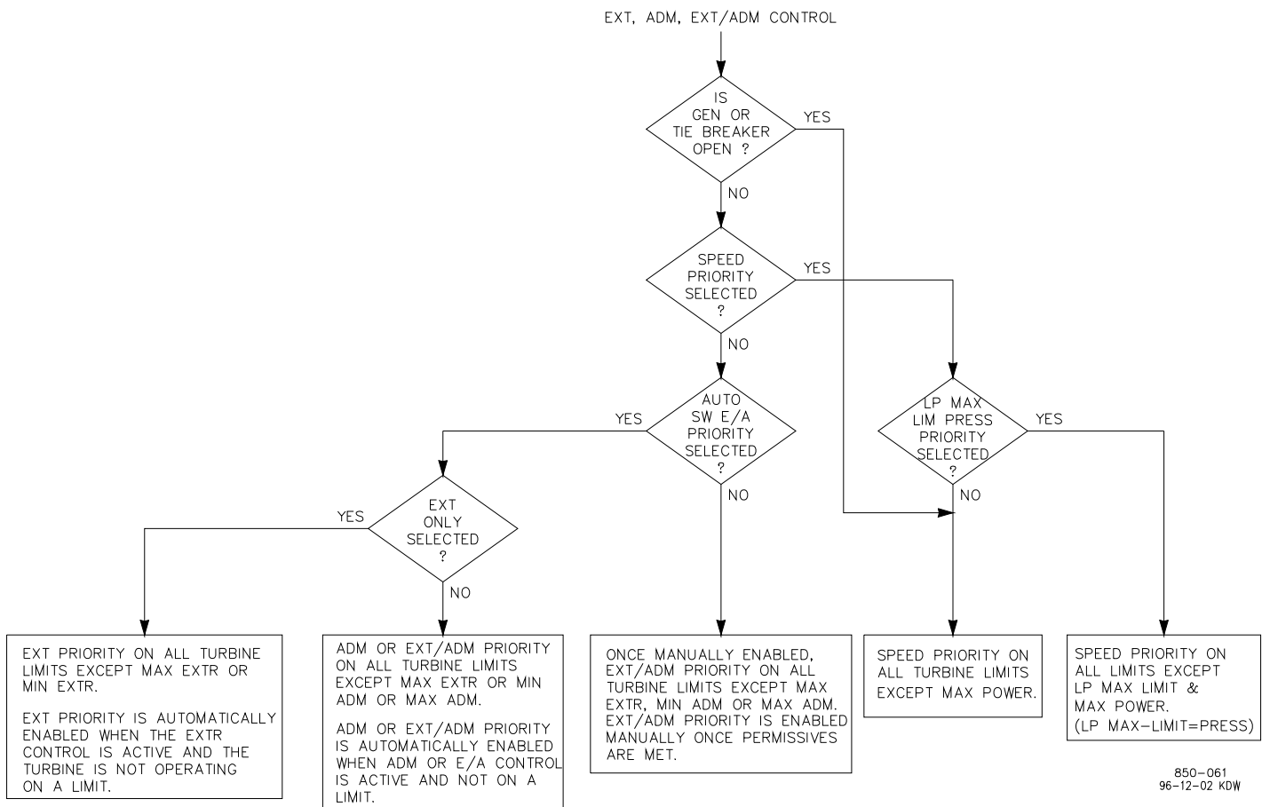
Figure 5-16. Priority Flow Diagram
