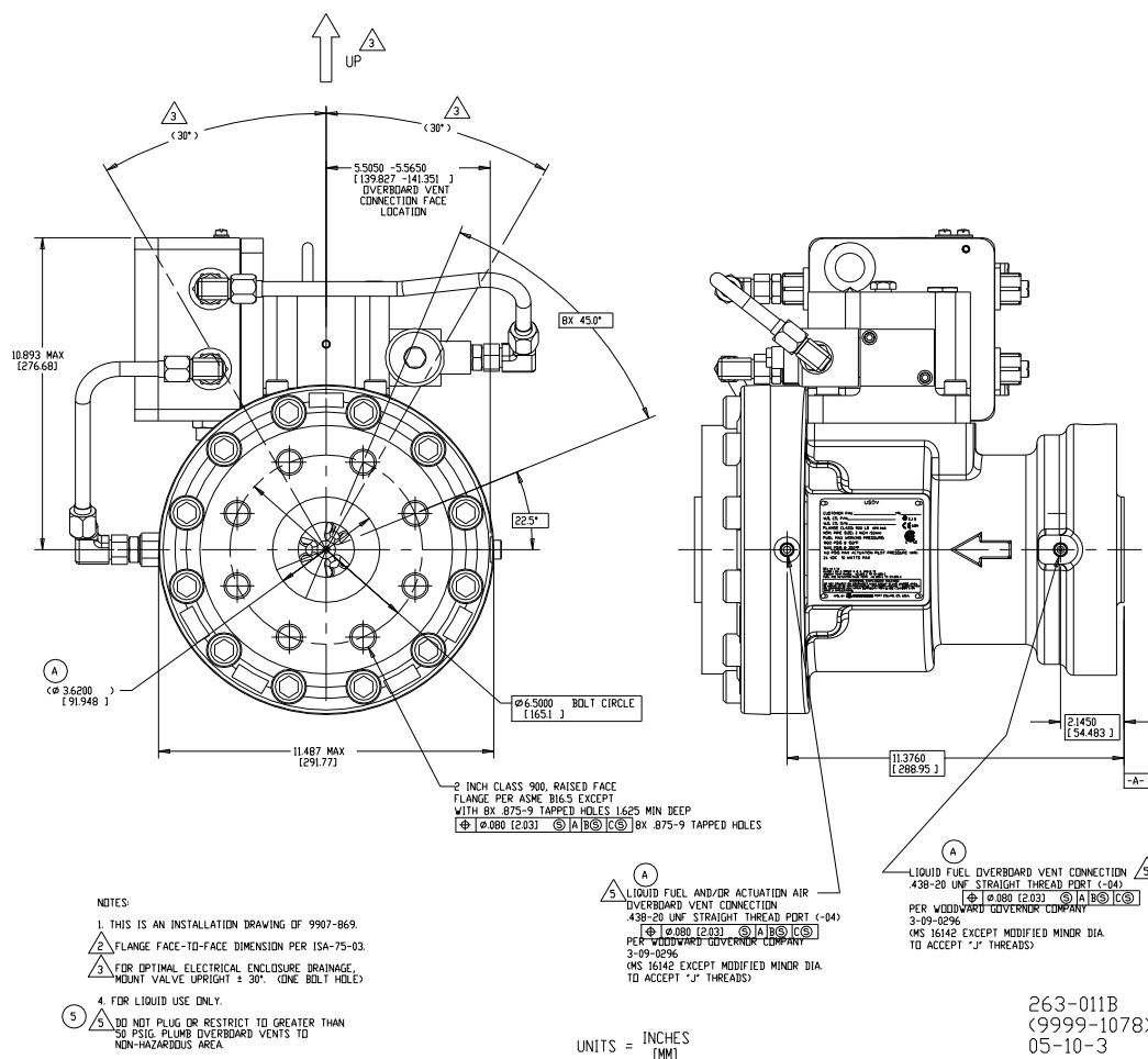
Figure 1-2b. Outline Drawing of 2 inch USOV
