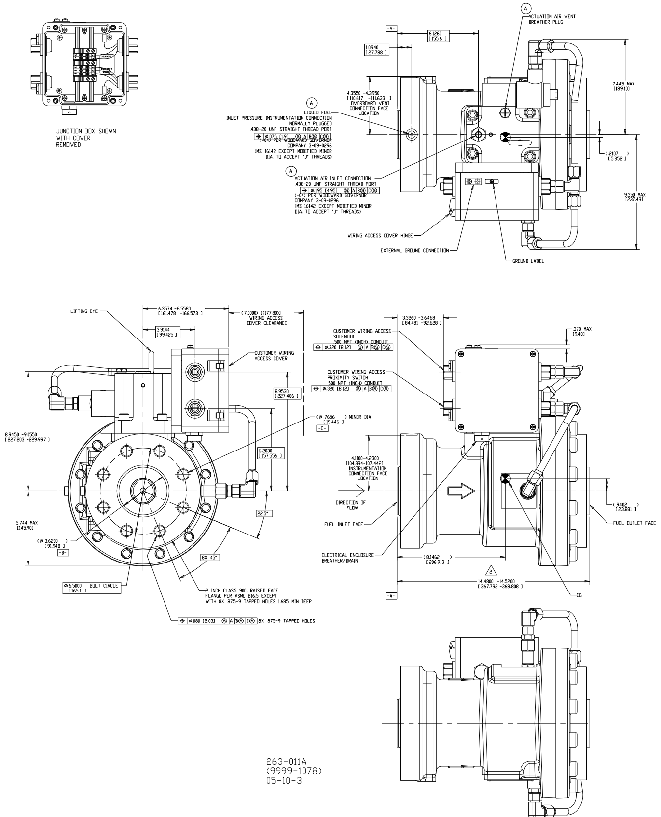
Figure 1-2a. Outline Drawing of 2 inch USOV
