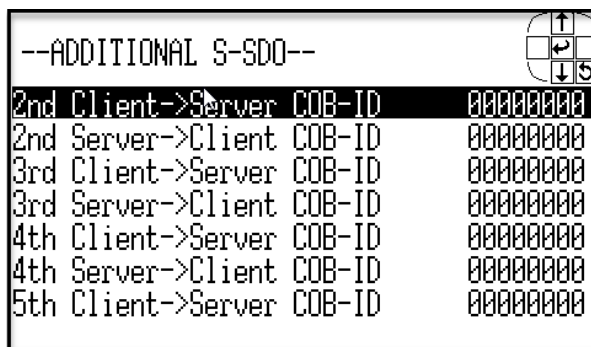
Figure 6-6: Display screen - configure Server SDOs
