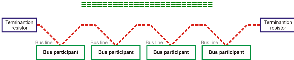
Figure 1-3: CAN bus topology
