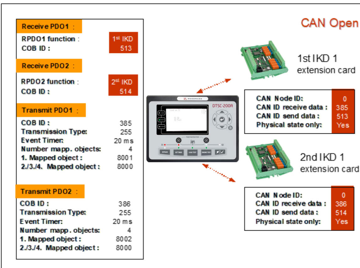
Figure 4-5: CANopen interface - expansion with two IKD 1
