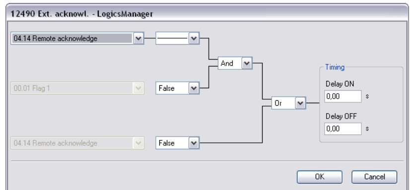
Figure 6-1: Display screen - Ext. acknowledge
