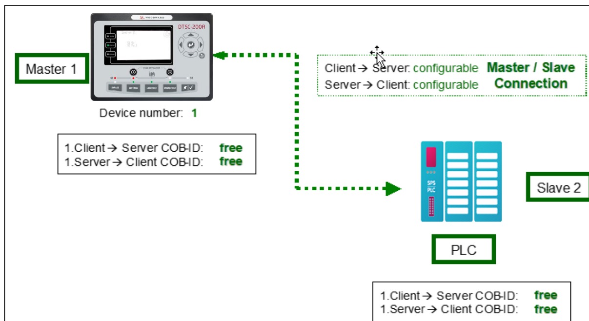
Figure 4-1: CANopen interface - overview
