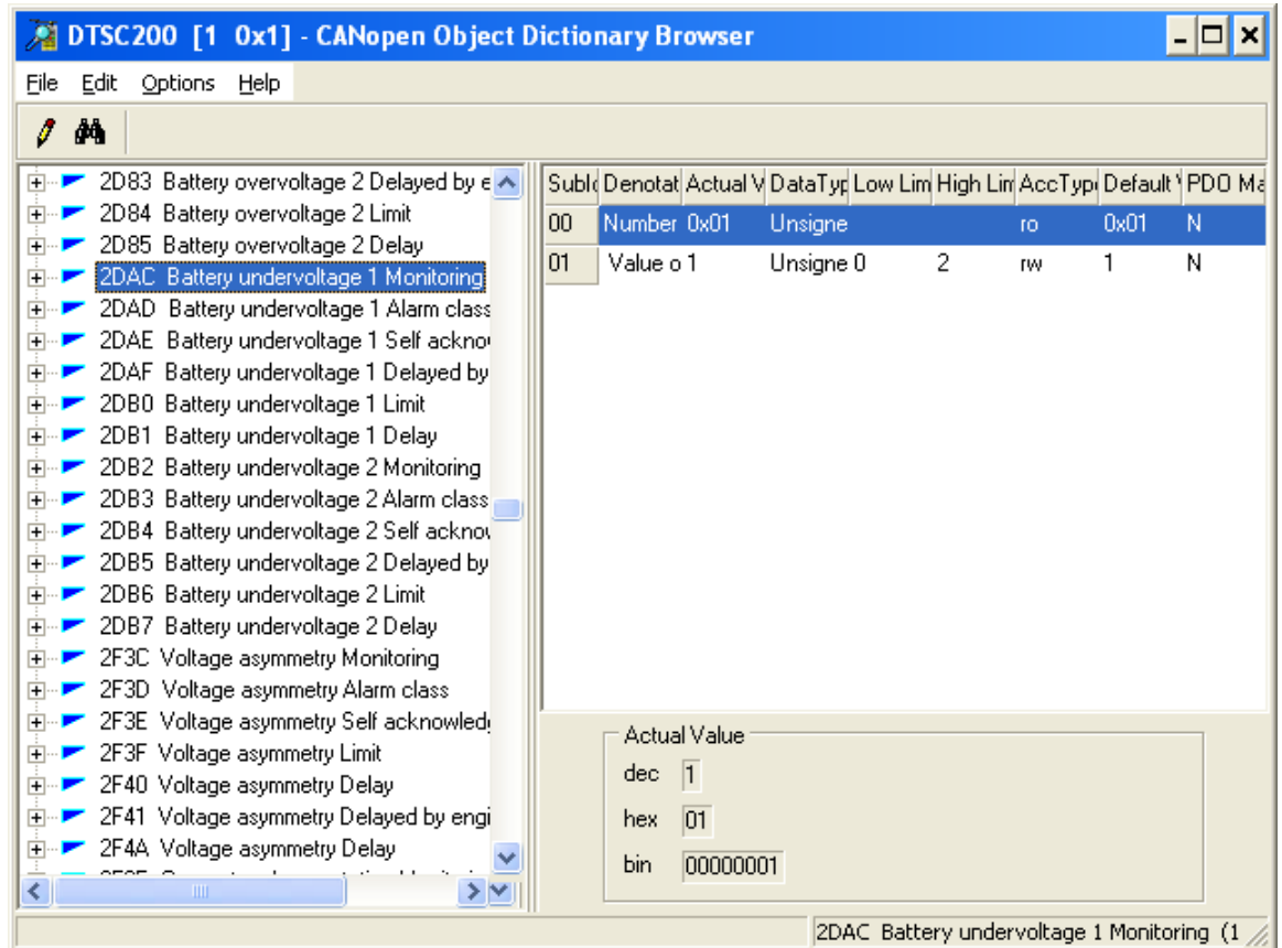
Figure 4-2: CANopen interface - CANopen configuration software
