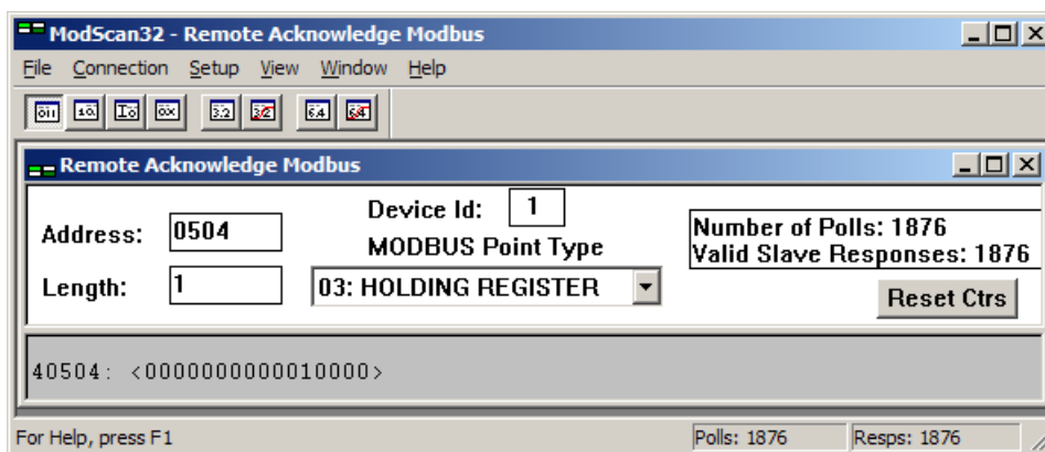
Figure 6-8: Modbus - remote control parameter 503
