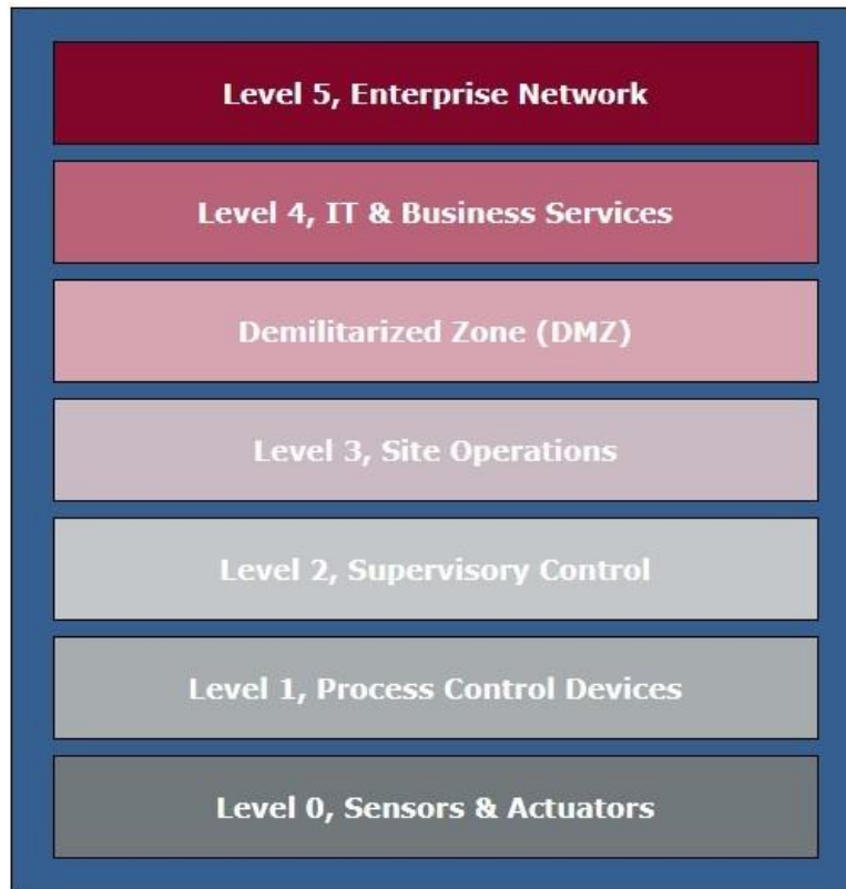
Figure 1-1. Purdue Model
